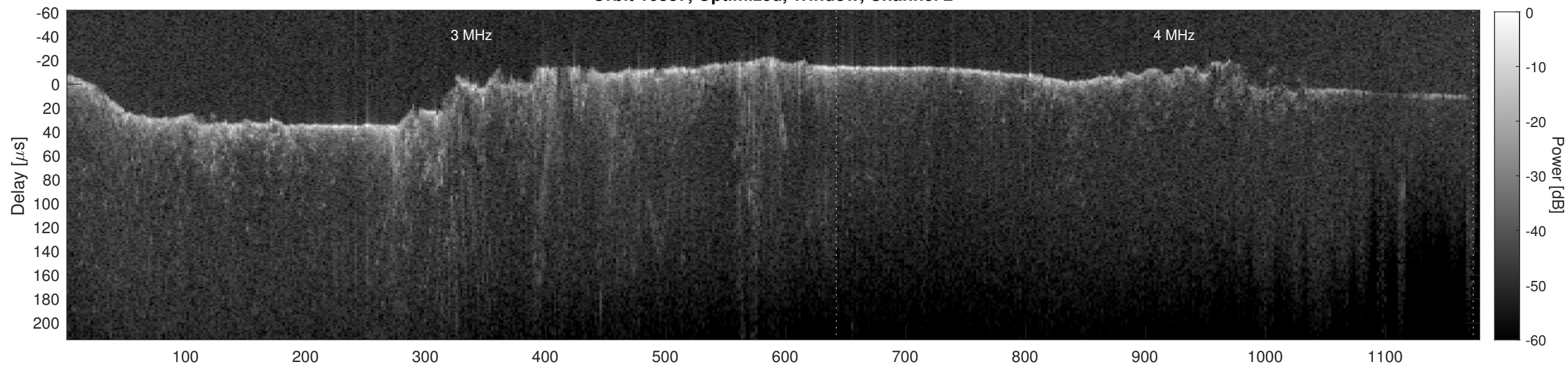
Orbit 10337, Cluttergram
