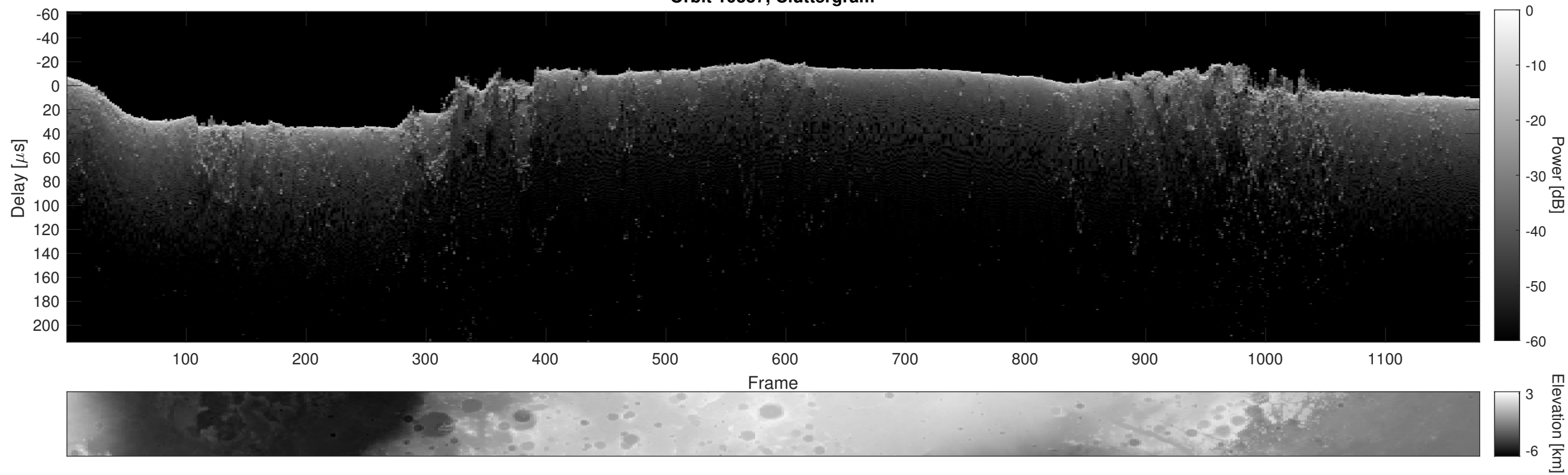
Orbit 10337, Cluttergram
