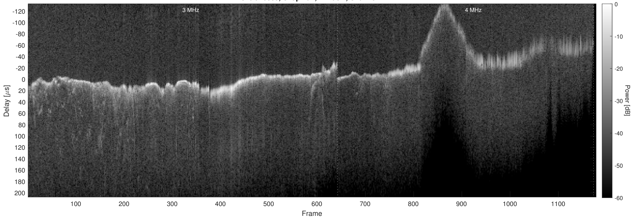
Orbit 10339, Chapman, Window, Channel 2
