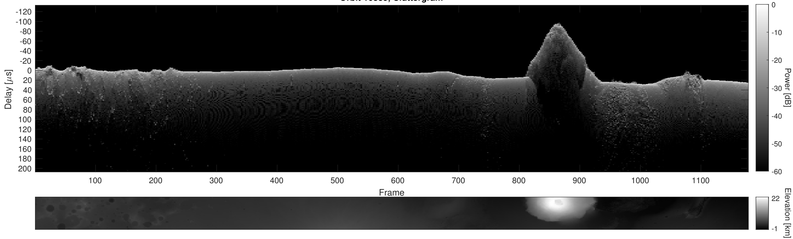
Orbit 10339, Cluttergram
