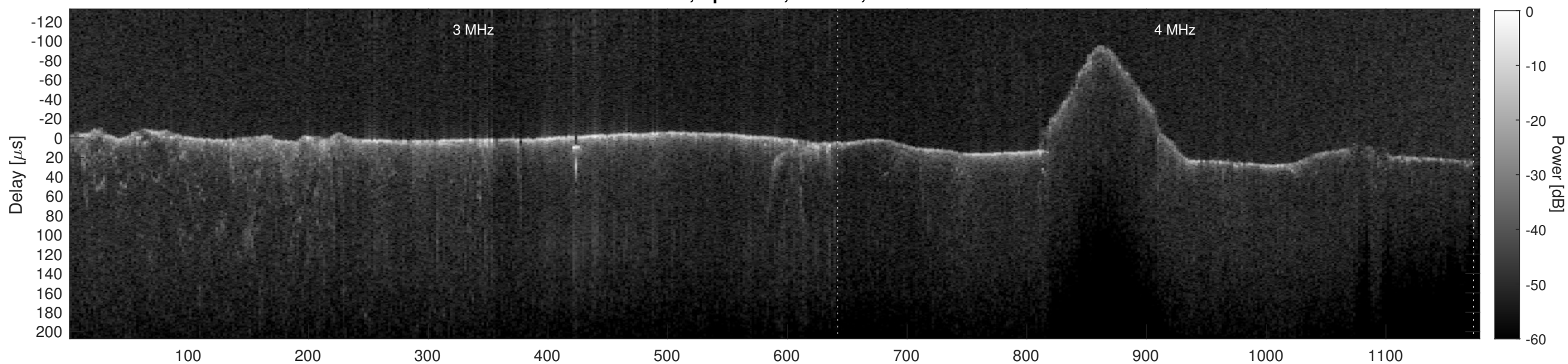
Orbit 10339, Cluttergram
