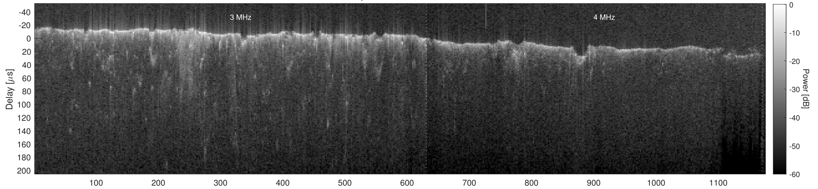
Orbit 10341, Cluttergram
