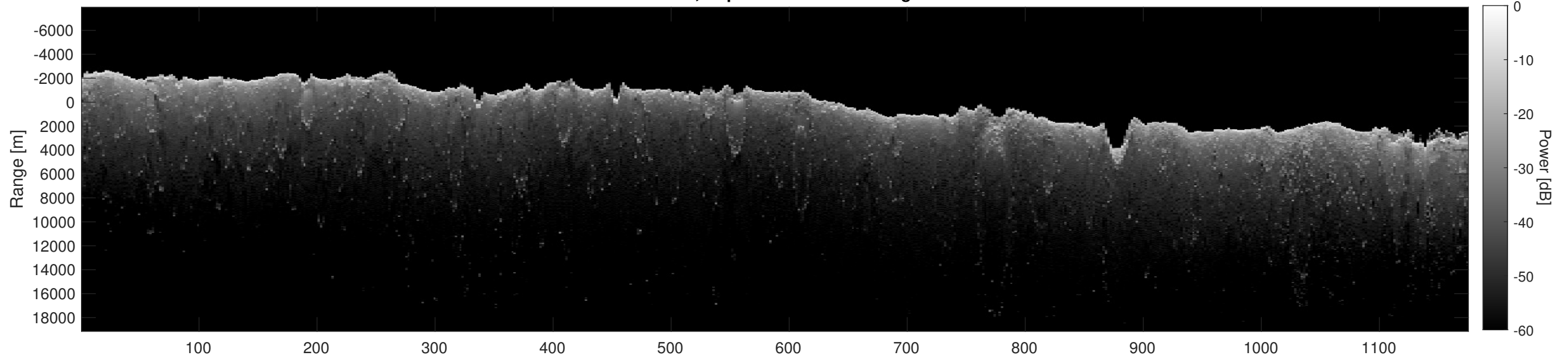
Orbit 10341, Depth-Corrected Cluttergram
