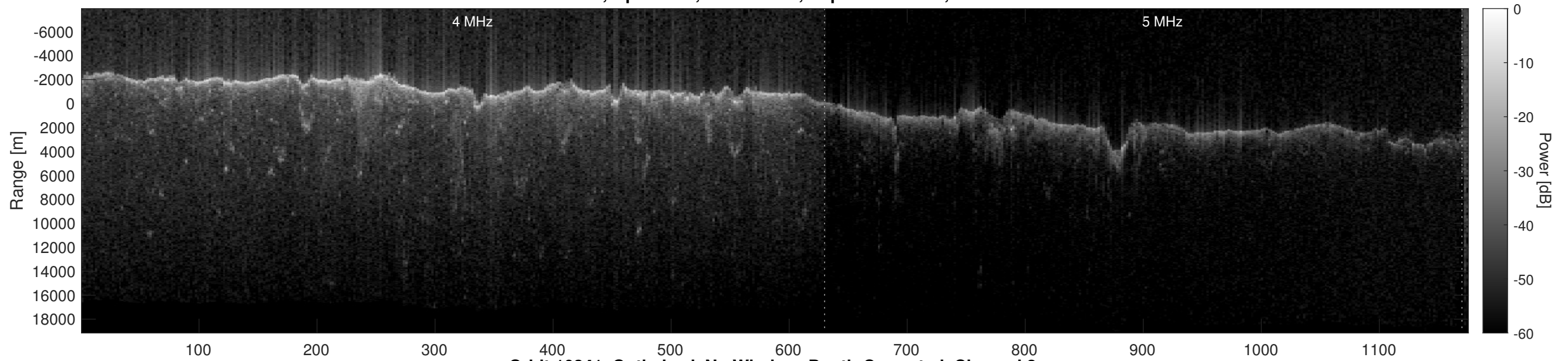
Orbit 10341, Optimized, No Window, Depth-Corrected, Channel 2
