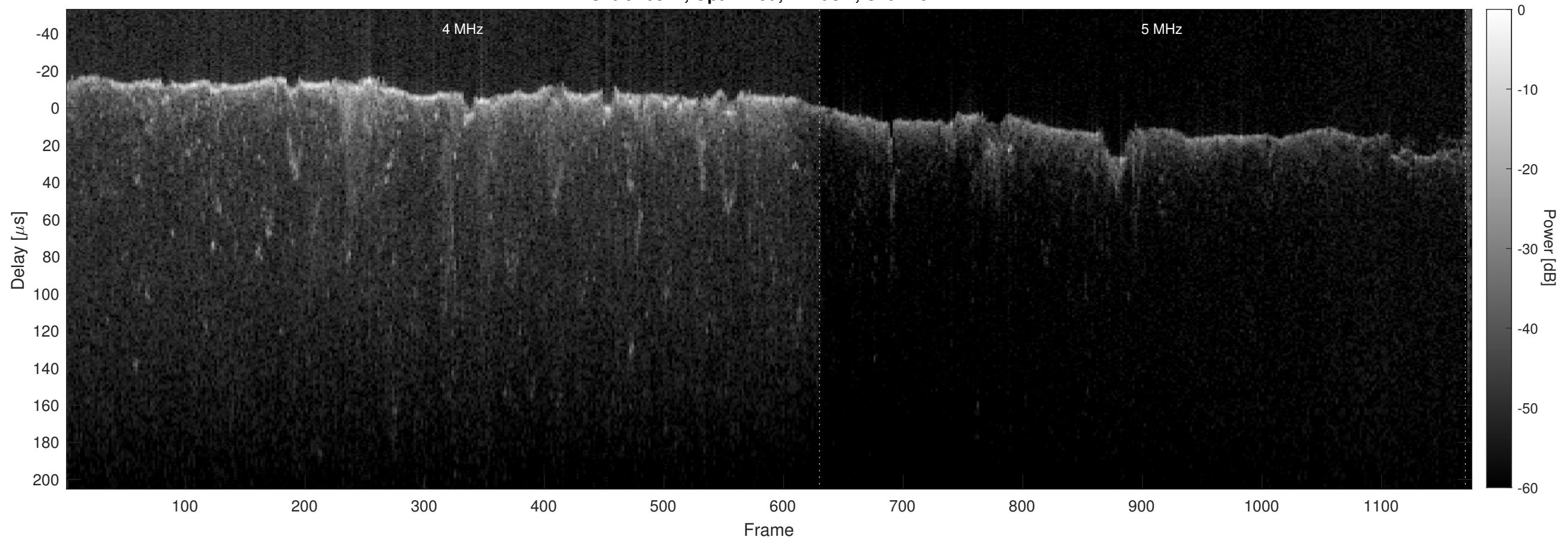
Orbit 10341, Optimized, Window, Channel 2
