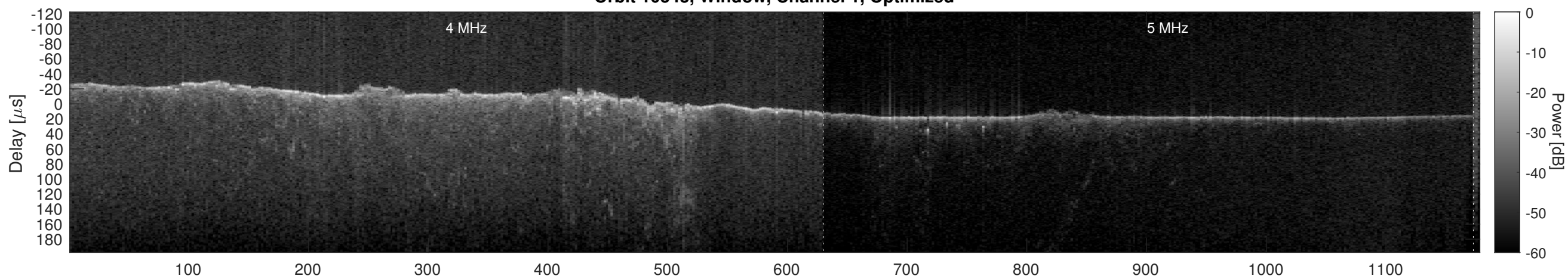
Orbit 10343, Cluttergram
