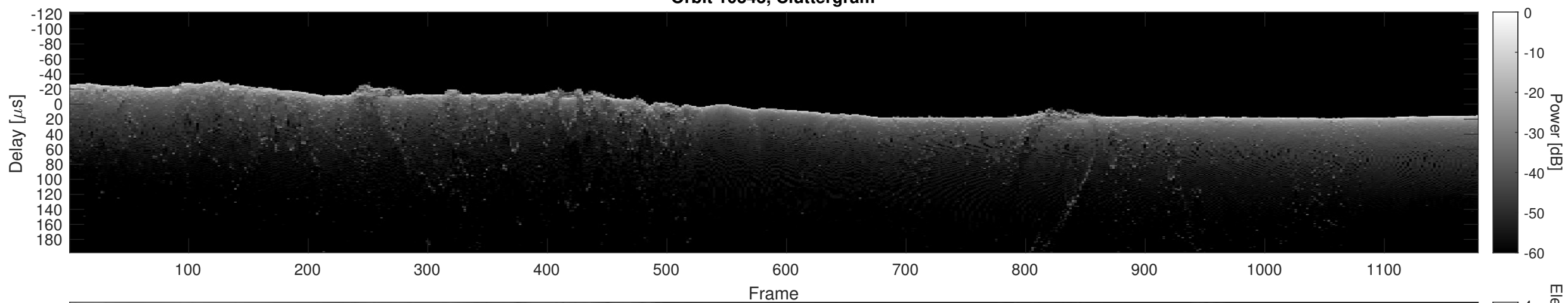
Orbit 10343, Cluttergram
