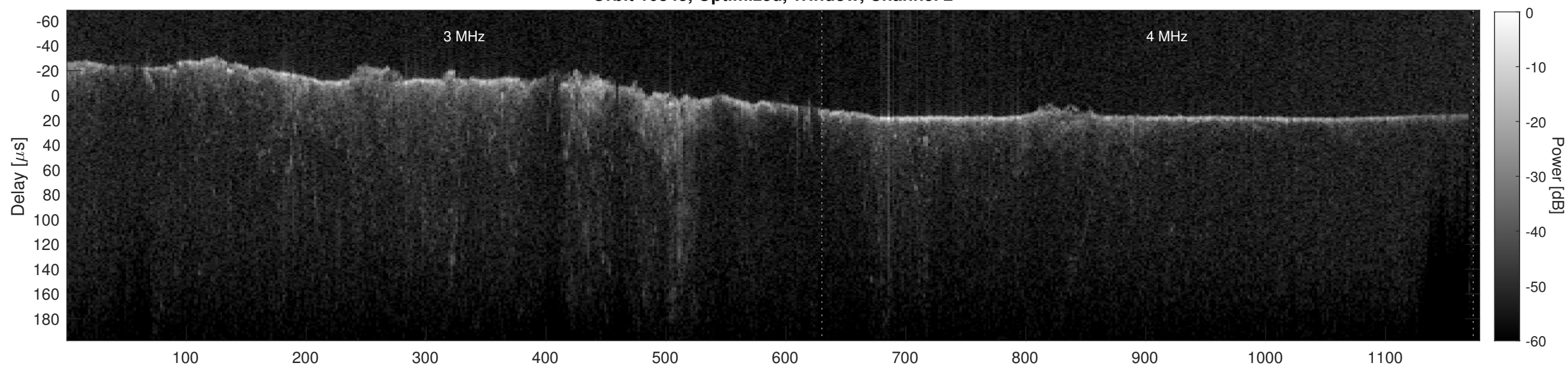
Orbit 10343, Cluttergram
