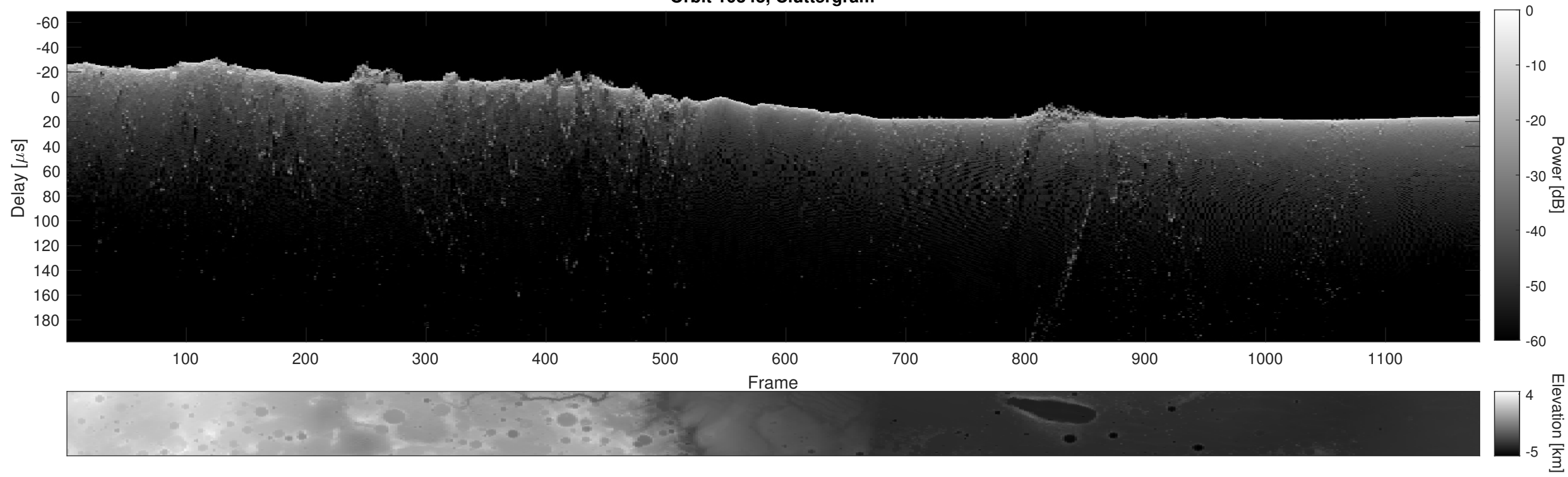
Orbit 10343, Cluttergram
