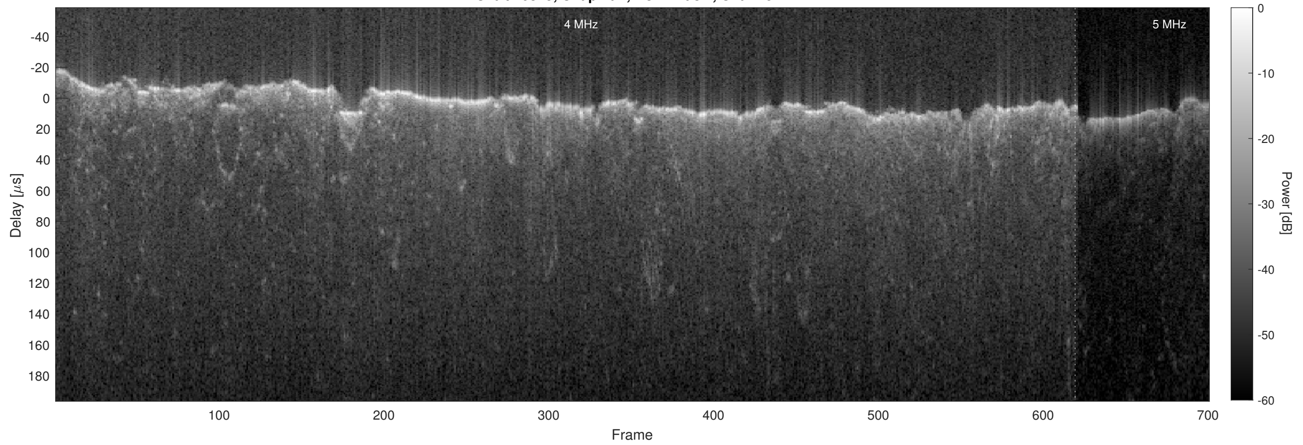
Orbit 10345, Chapman, No Window, Channel 2
