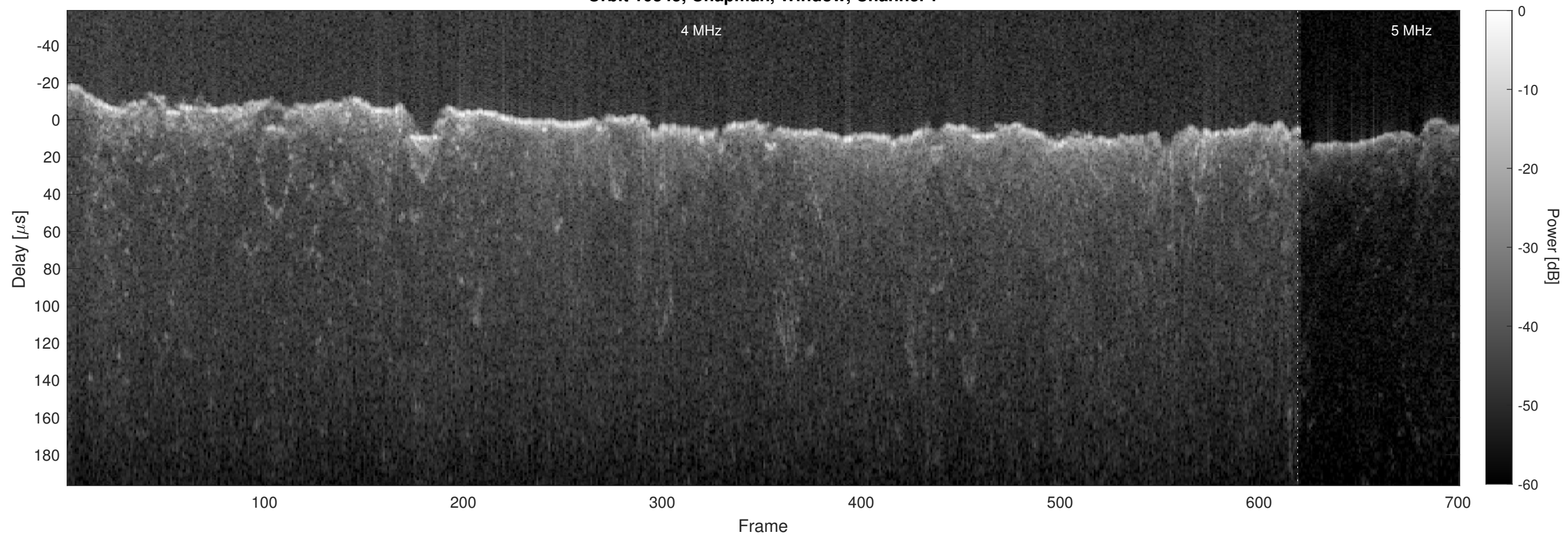
Orbit 10345, Chapman, Window, Channel 2
