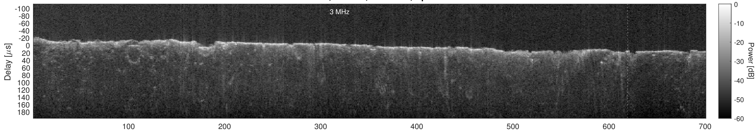
Orbit 10345, Cluttergram
