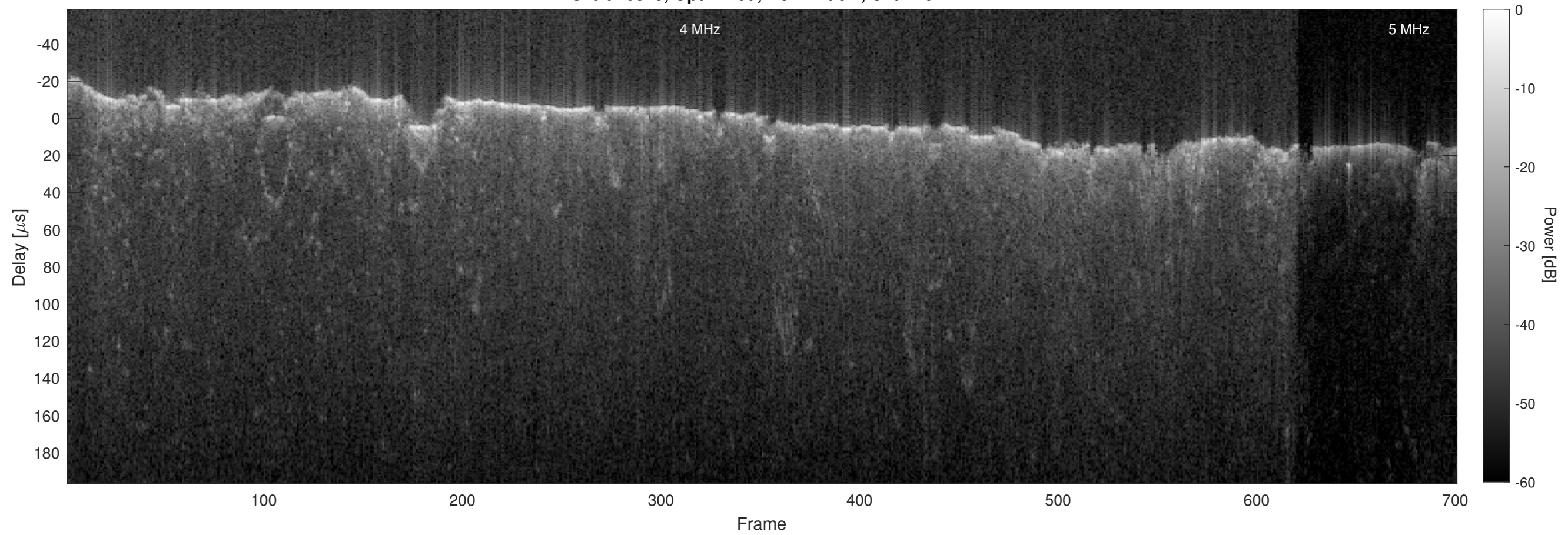
Orbit 10345, Optimized, No Window, Channel 2
