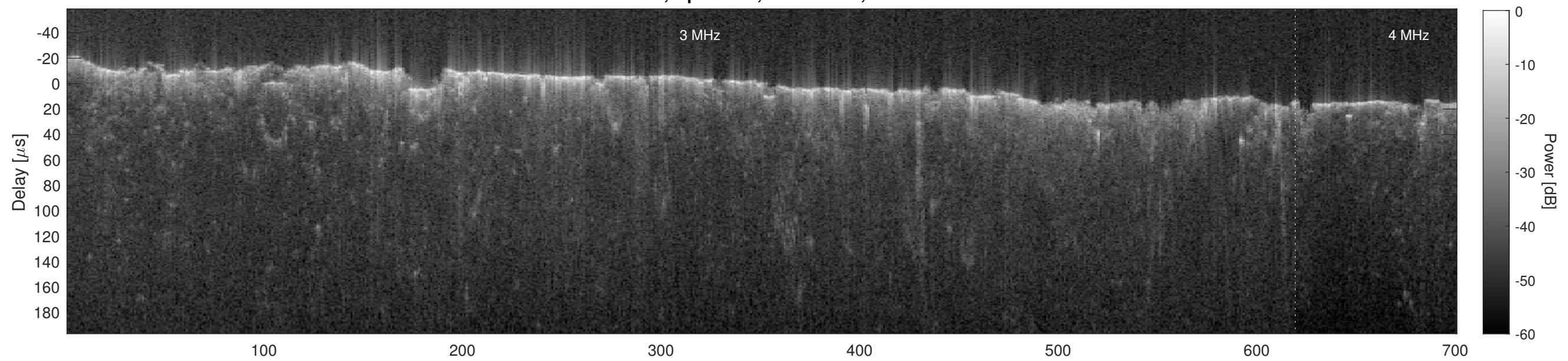
Orbit 10345, Cluttergram
