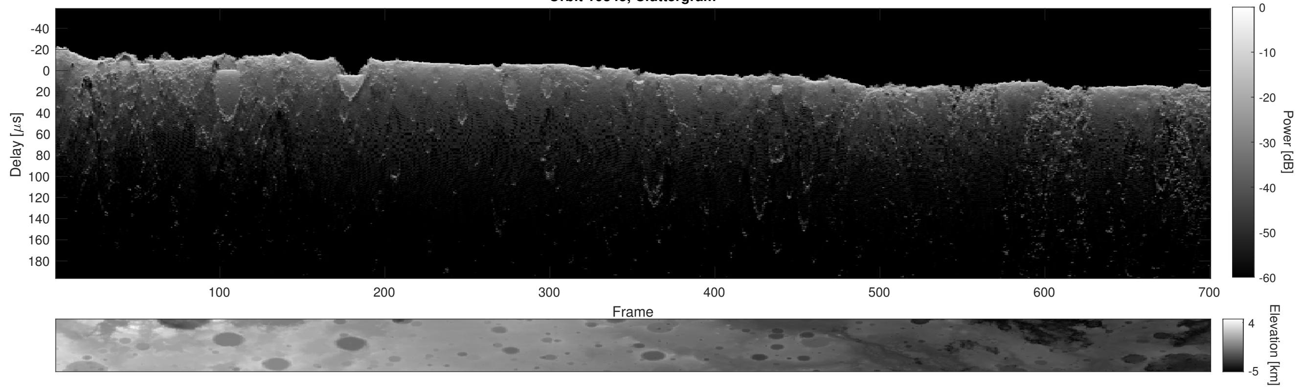
Orbit 10345, Cluttergram
