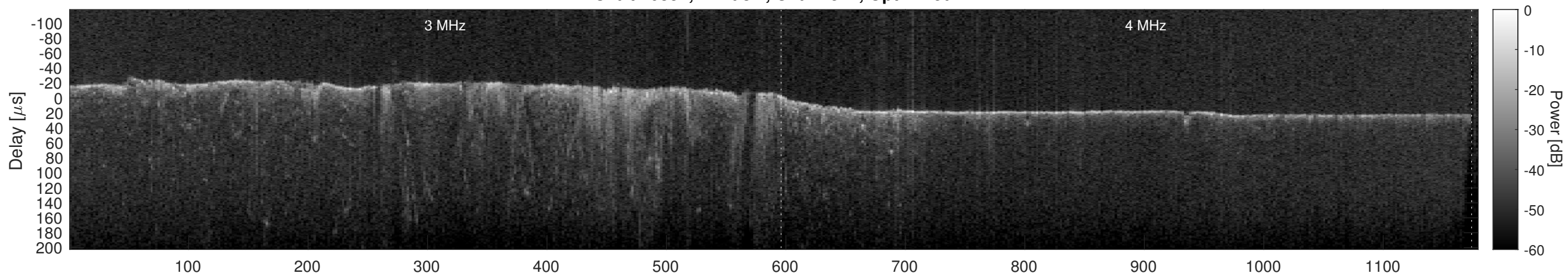
Orbit 10354, Cluttergram
