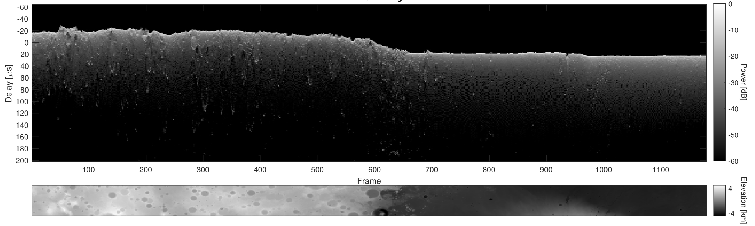
Orbit 10354, Cluttergram
