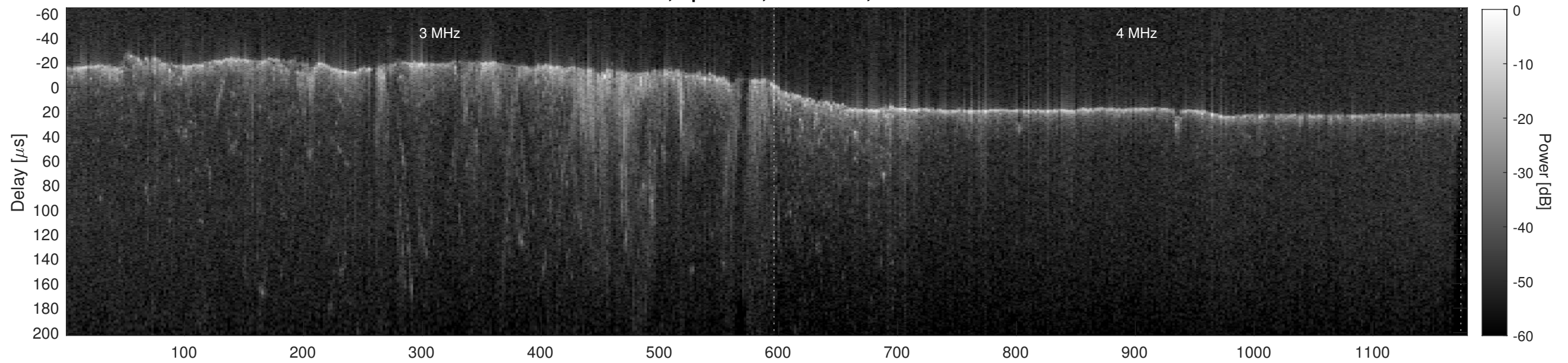
Orbit 10354, Cluttergram
