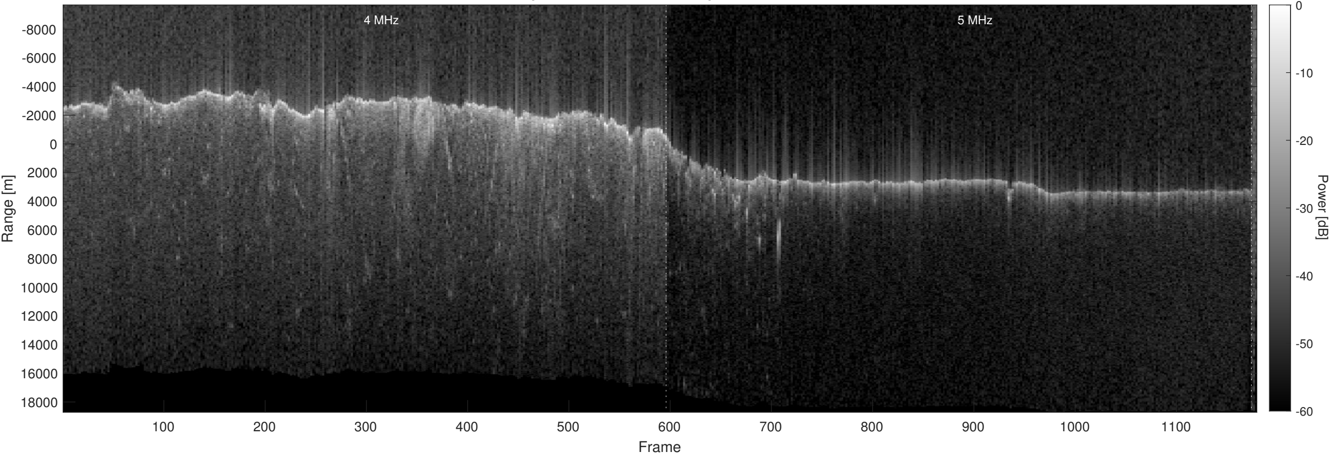
Orbit 10354, Optimized, No Window, Depth-Corrected, Channel 2
