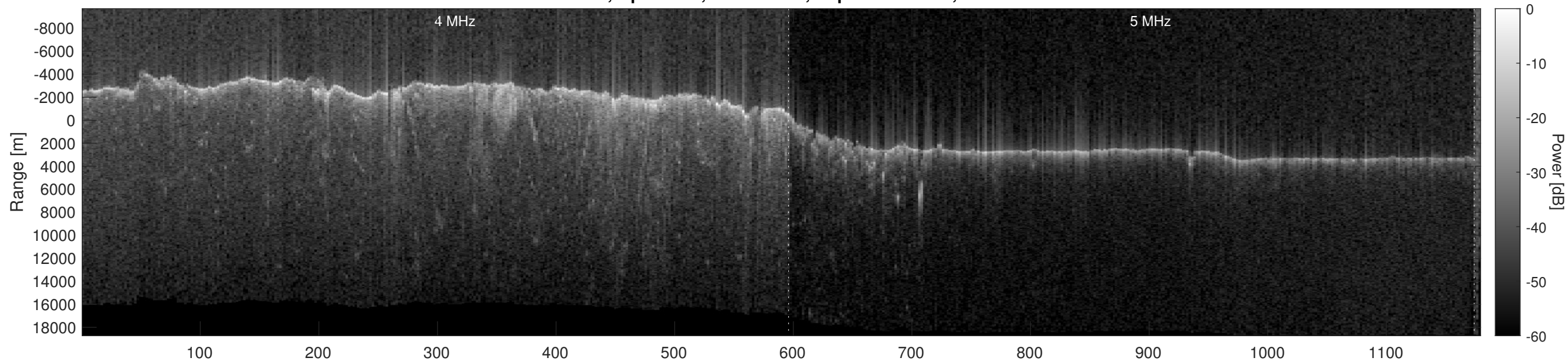
Orbit 10354, Optimized, No Window, Depth-Corrected, Channel 2
