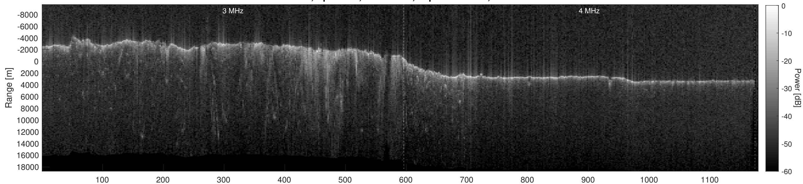
Orbit 10354, Depth-Corrected Cluttergram
