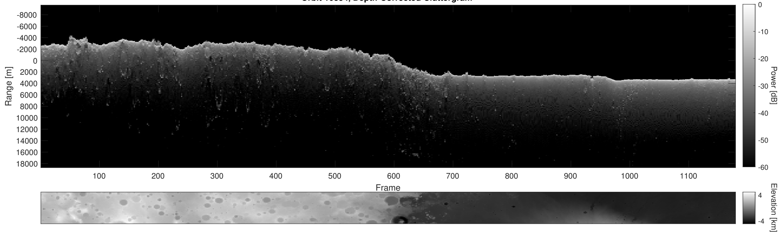
Orbit 10354, Depth-Corrected Cluttergram
