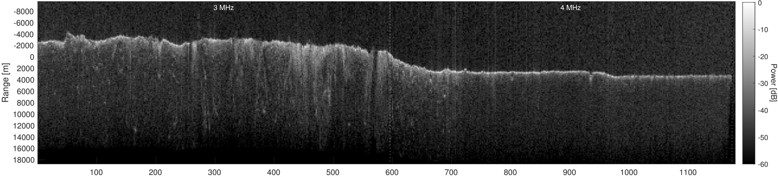
Orbit 10354, Depth-Corrected Cluttergram
