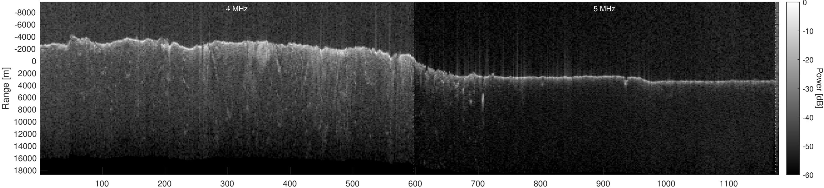
Orbit 10354, Optimized, Window, Depth-Corrected, Channel 2
