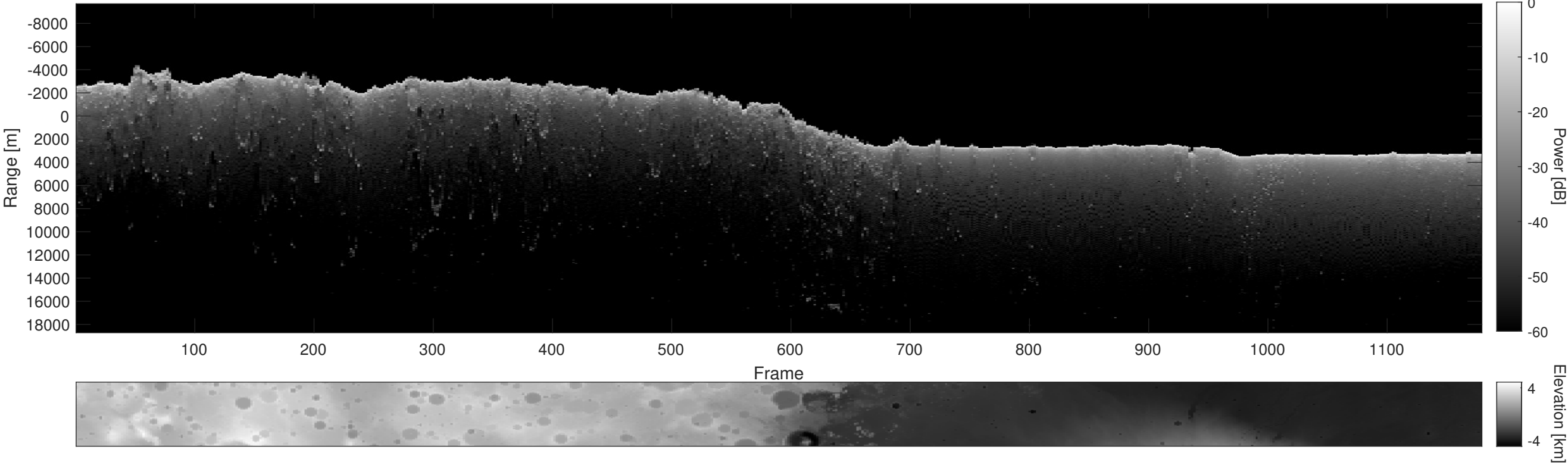
Orbit 10354, Depth-Corrected Cluttergram
