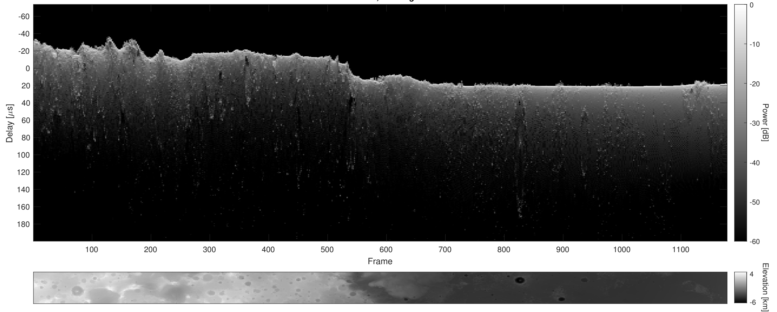
Orbit 10357, Cluttergram
