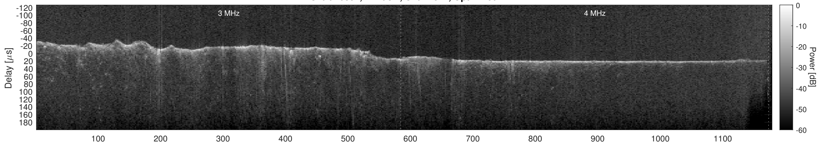
Orbit 10357, Cluttergram
