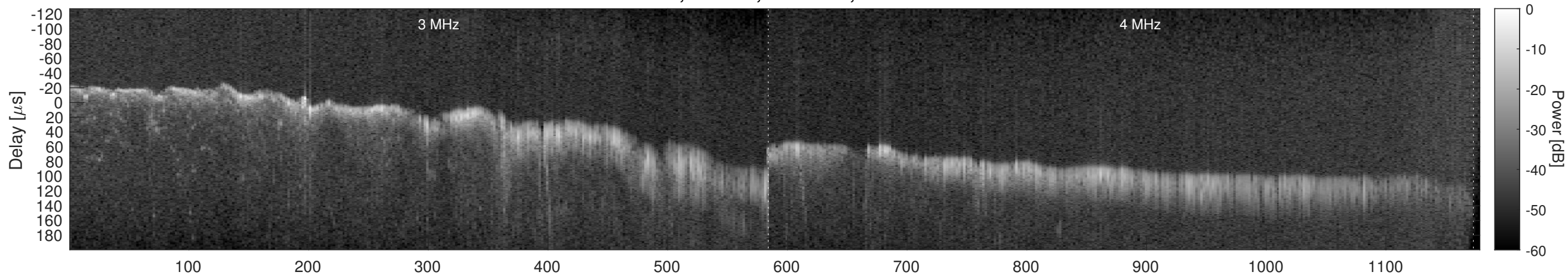
Orbit 10357, Window, Channel 2, Chapman
