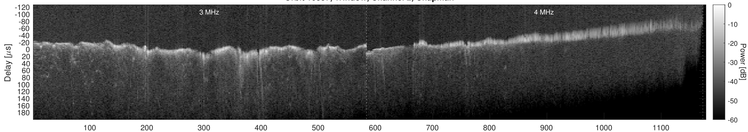
Orbit 10357, Window, Channel 2, Optimized
