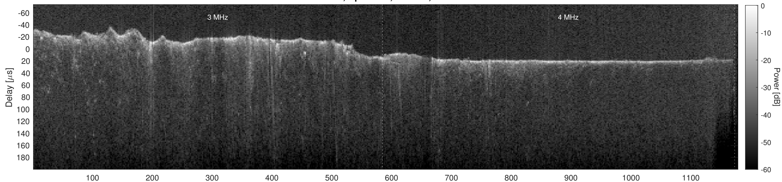
Orbit 10357, Cluttergram
