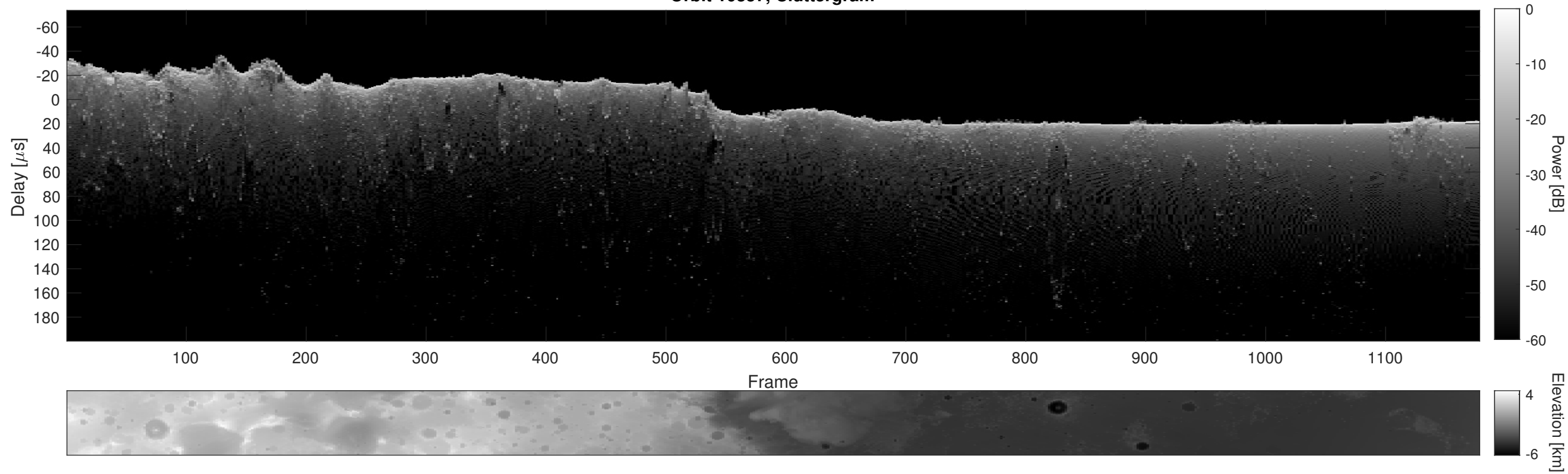
Orbit 10357, Cluttergram
