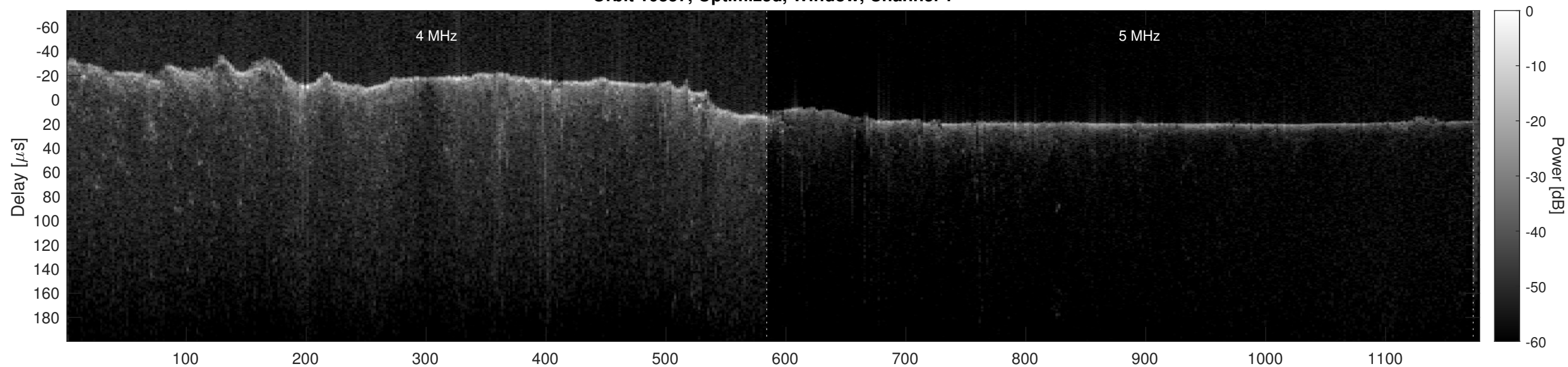
Orbit 10357, Optimized, Window, Channel 2
