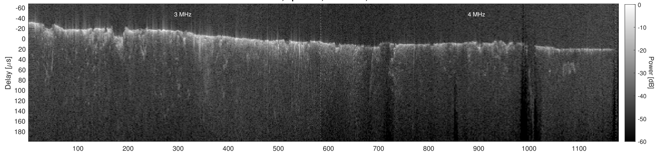
Orbit 10359, Cluttergram
