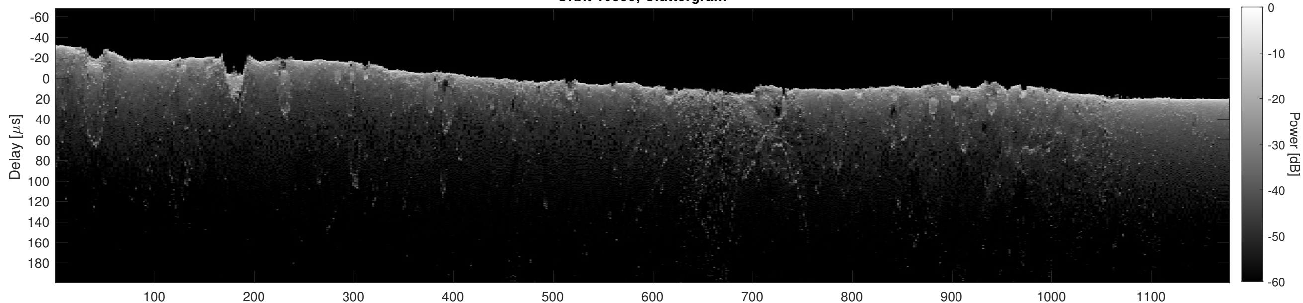
Orbit 10359, Cluttergram
