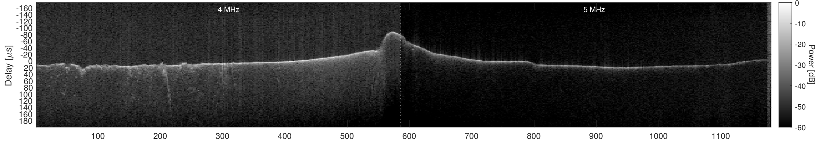
Orbit 10360, Cluttergram
