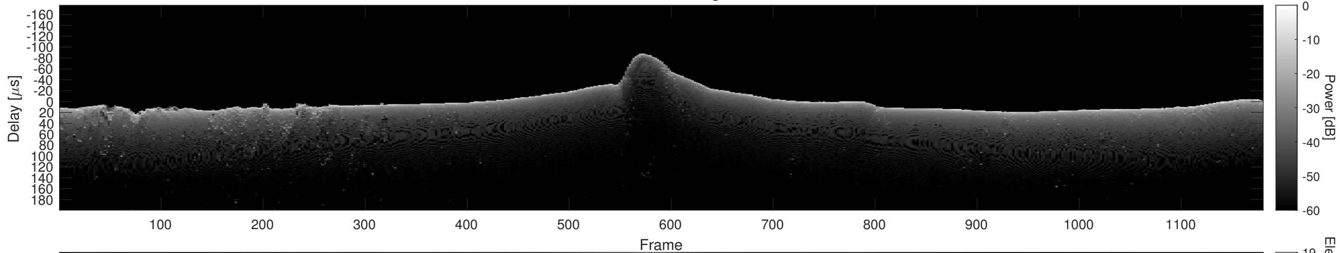
Orbit 10360, Cluttergram
