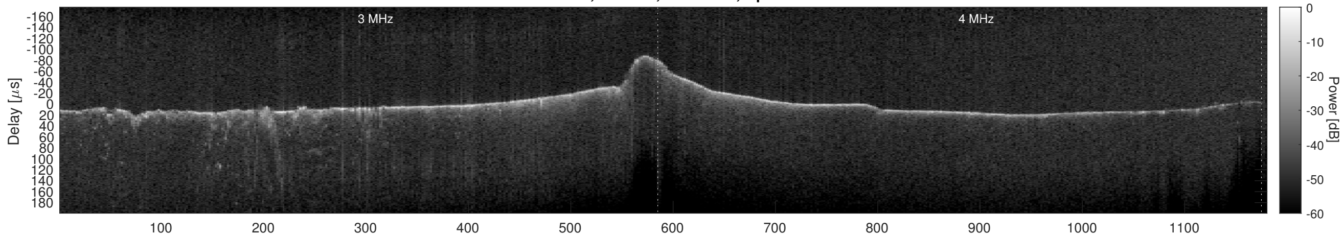
Orbit 10360, Cluttergram
