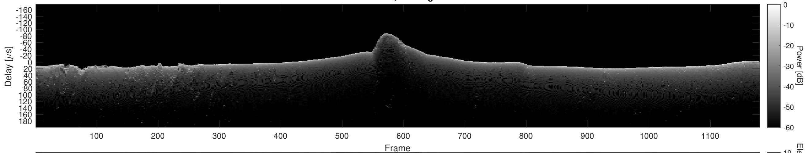
Orbit 10360, Cluttergram
