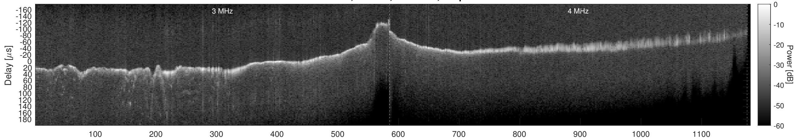
Orbit 10360, Window, Channel 2, Optimized
