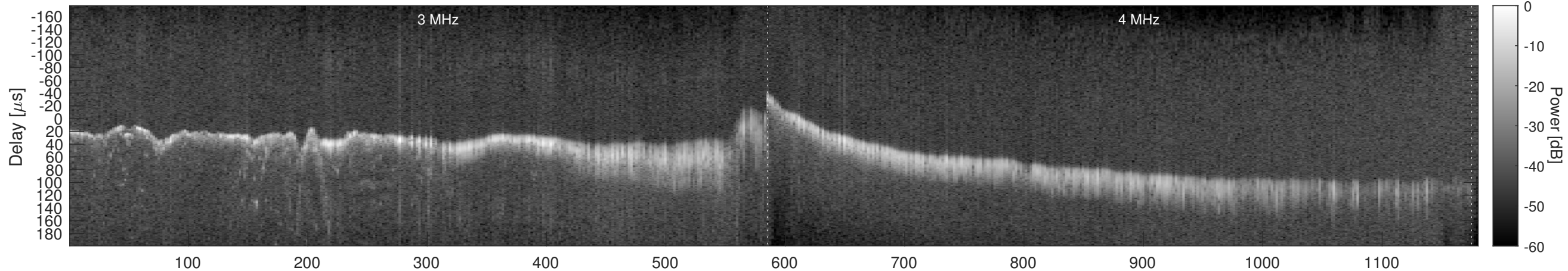
Orbit 10360, Window, Channel 2, Chapman
