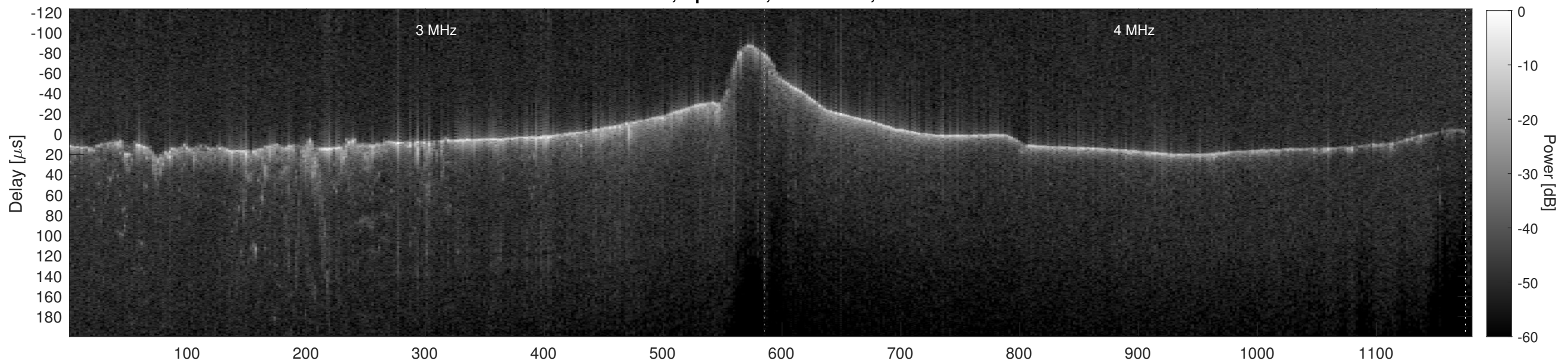
Orbit 10360, Cluttergram
