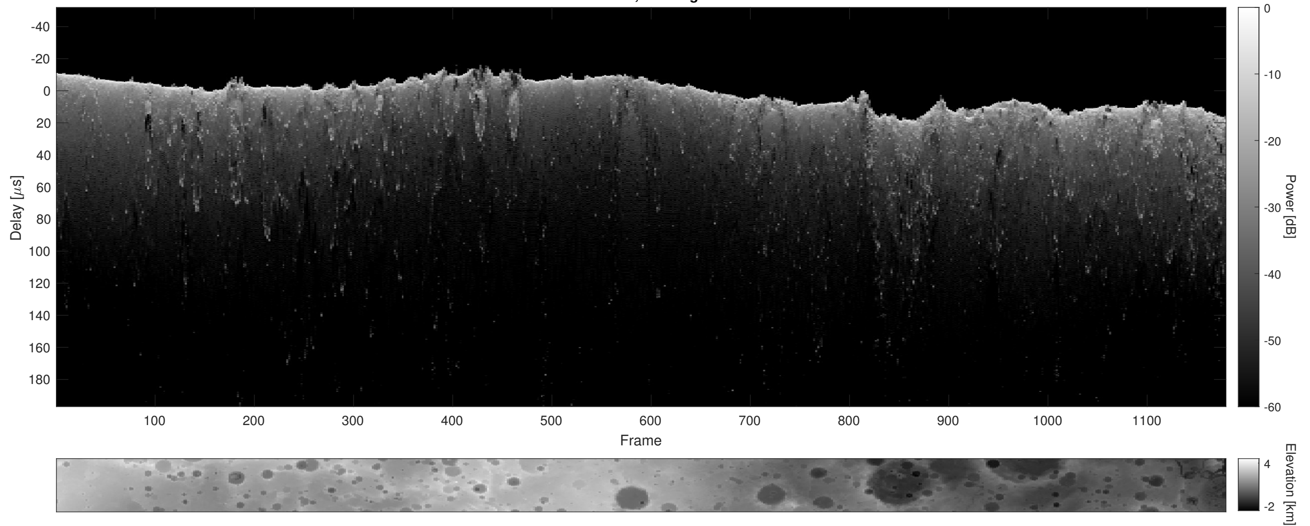
Orbit 10362, Cluttergram
