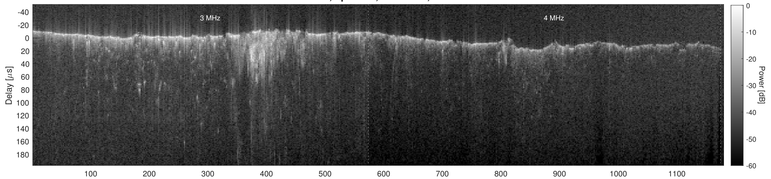
Orbit 10362, Cluttergram
