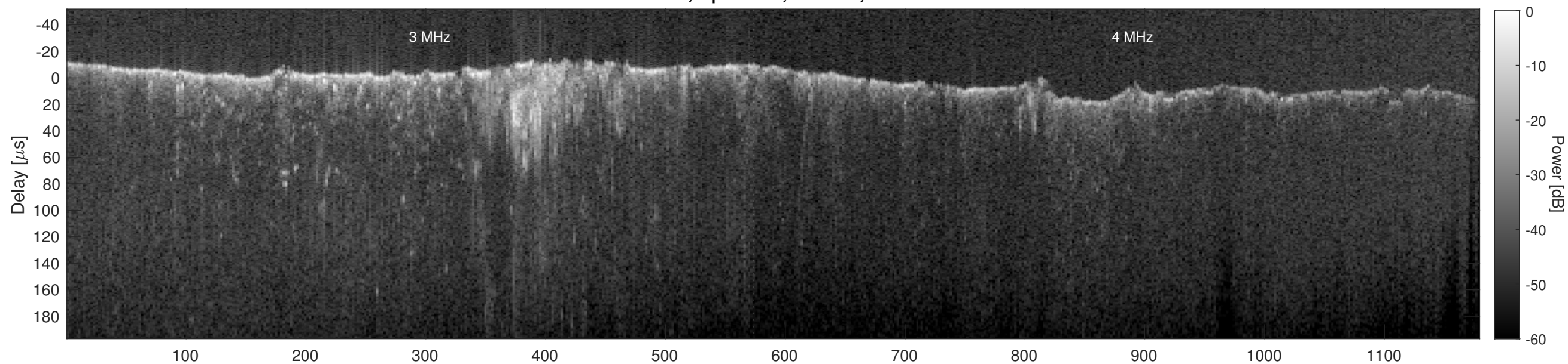
Orbit 10362, Cluttergram
