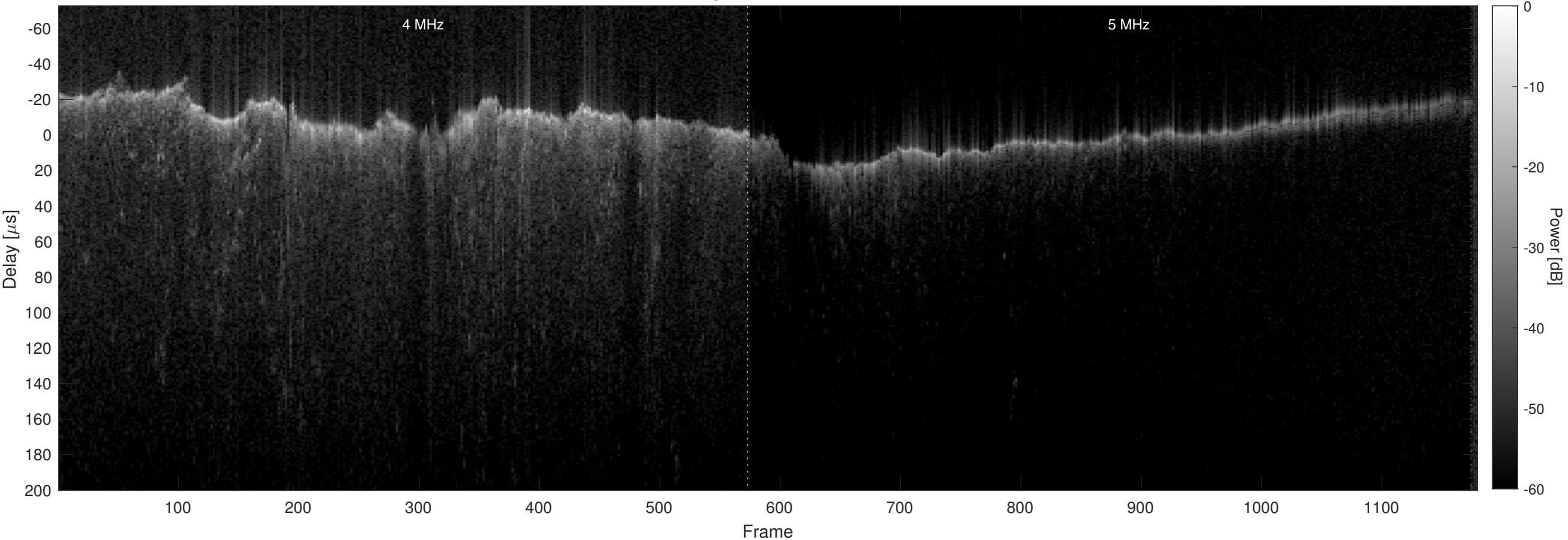
Orbit 10364, Chapman, No Window, Channel 2
