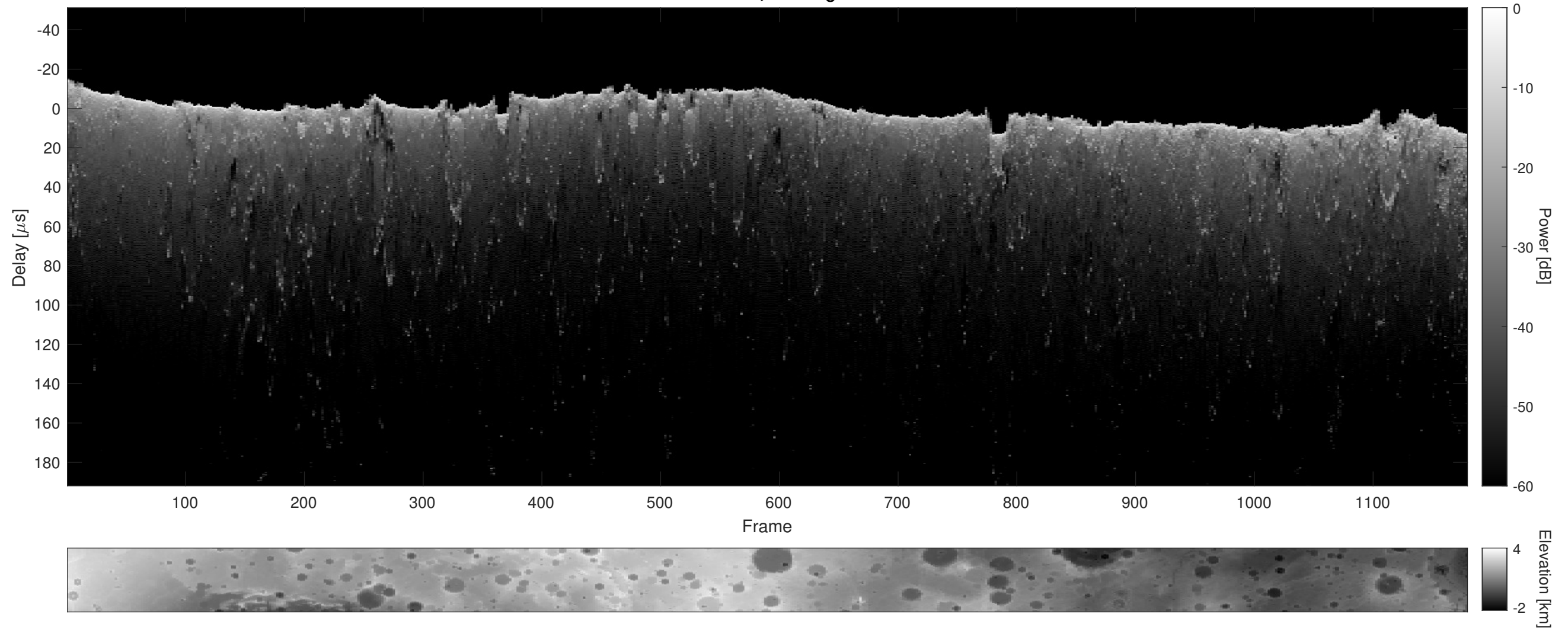
Orbit 10369, Cluttergram
