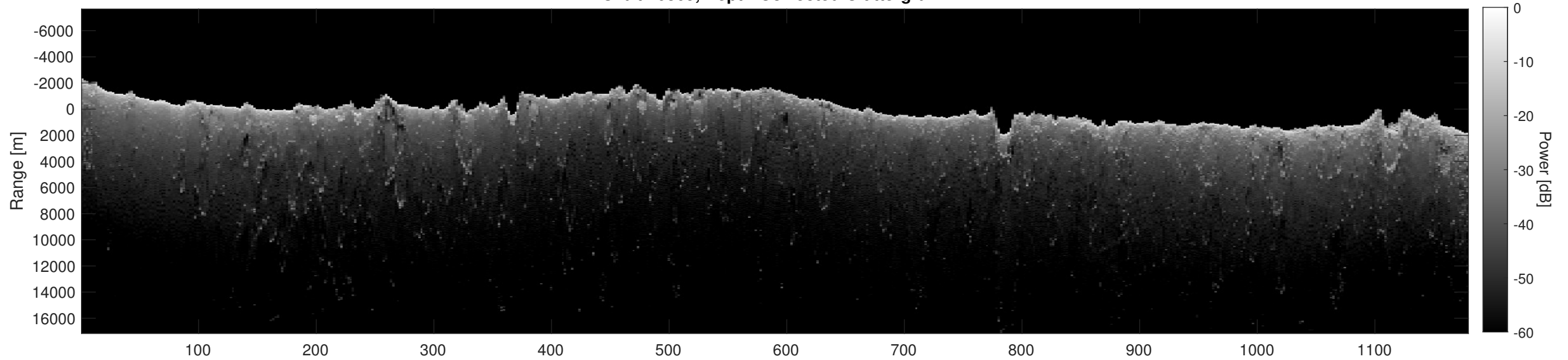
Orbit 10369, Depth-Corrected Cluttergram
