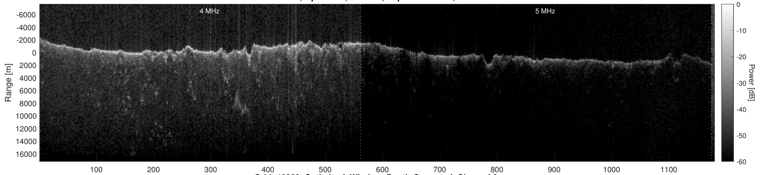
Orbit 10369, Optimized, Window, Depth-Corrected, Channel 2
