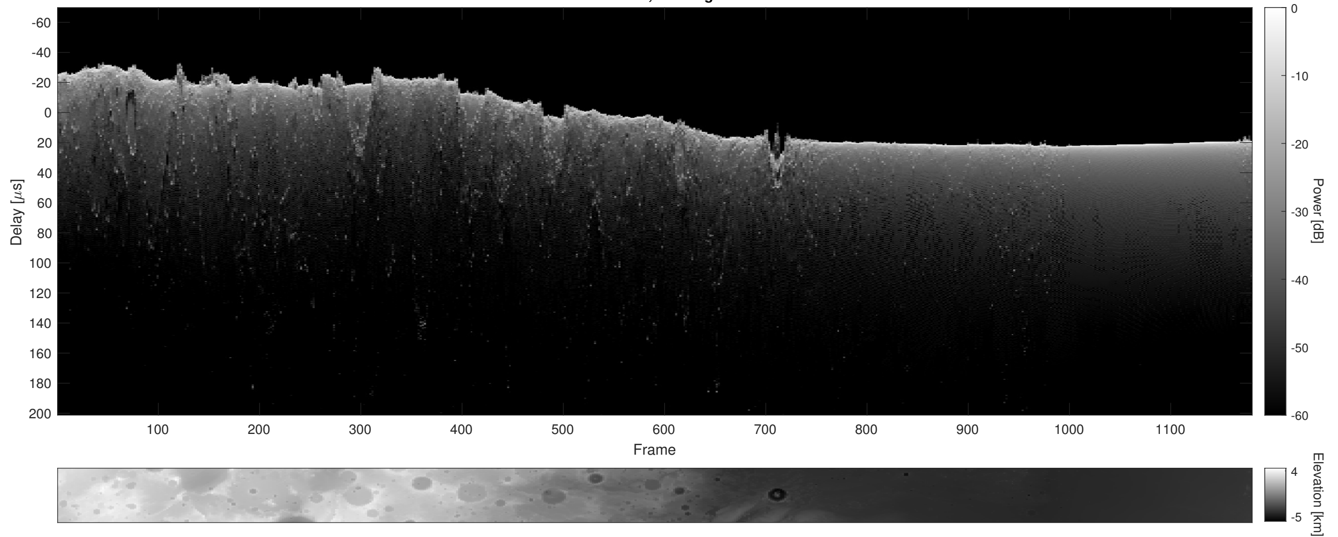
Orbit 10371, Cluttergram
