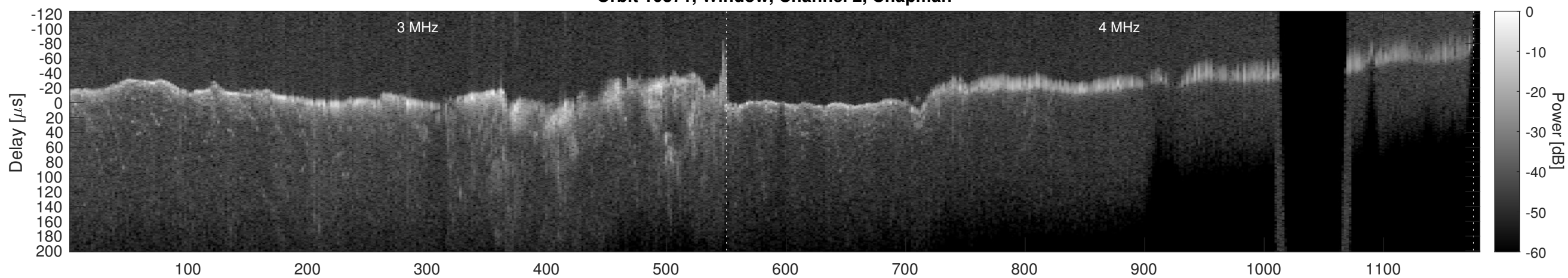
Orbit 10371, Window, Channel 2, Optimized
