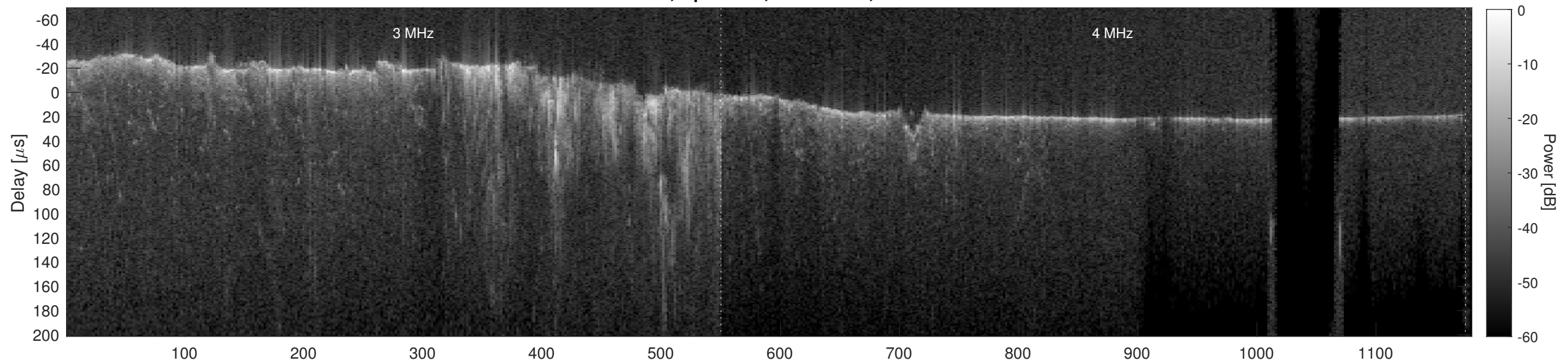
Orbit 10371, Cluttergram
