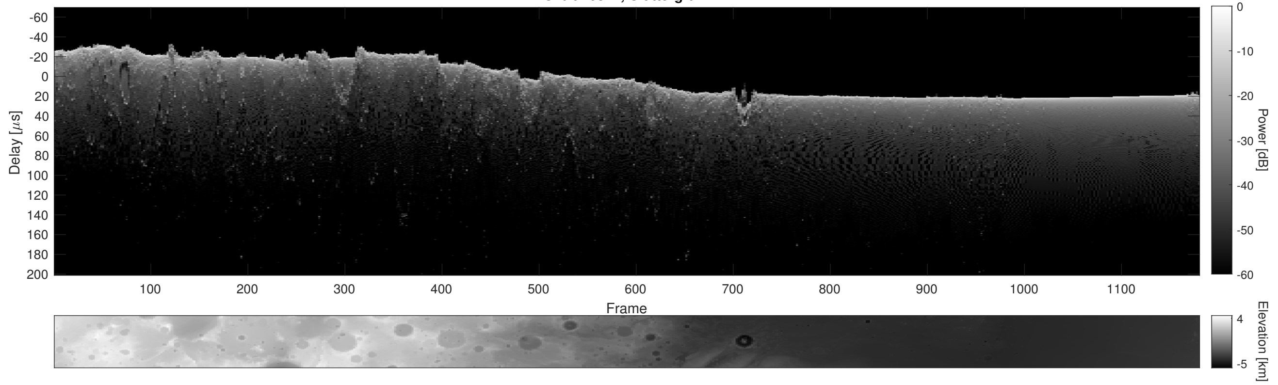
Orbit 10371, Cluttergram
