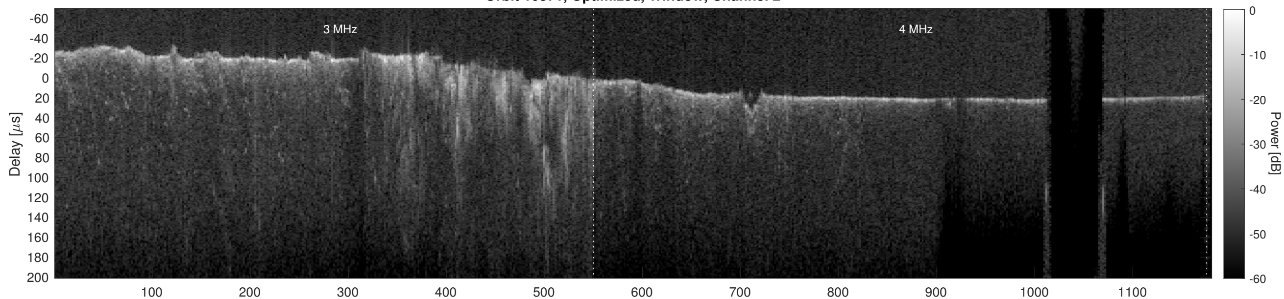
Orbit 10371, Cluttergram
