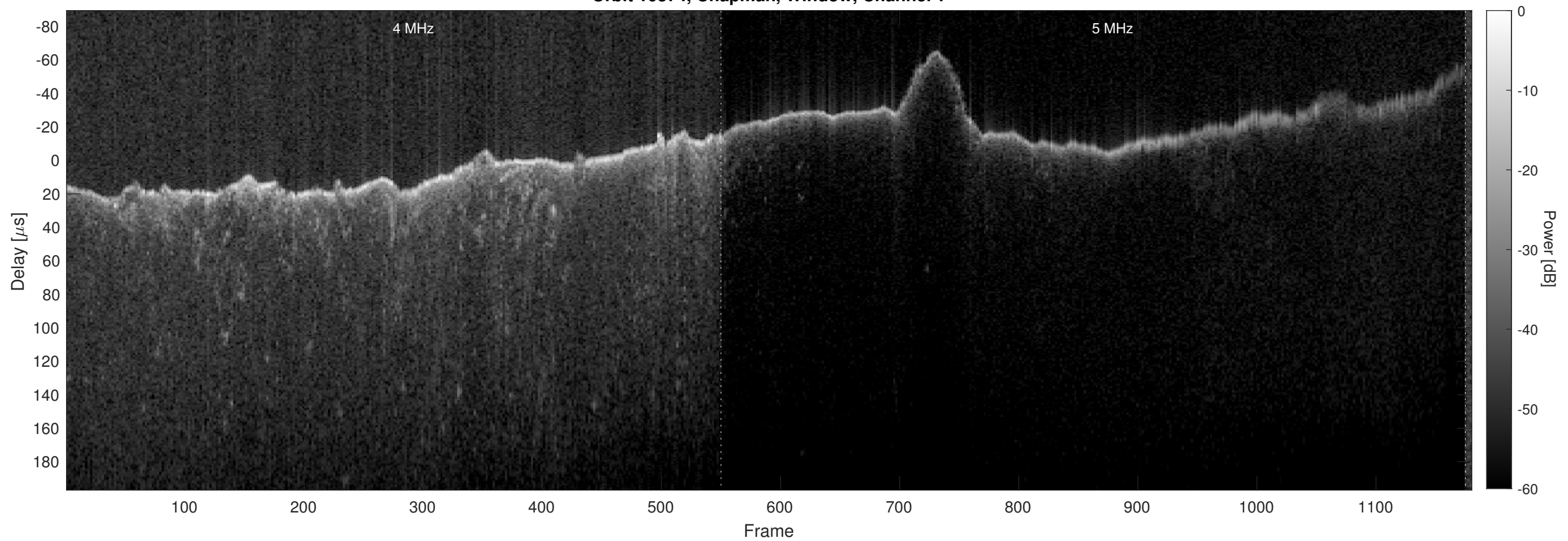
Orbit 10374, Chapman, Window, Channel 2
