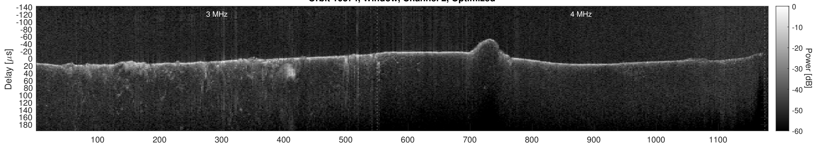
Orbit 10374, Cluttergram
