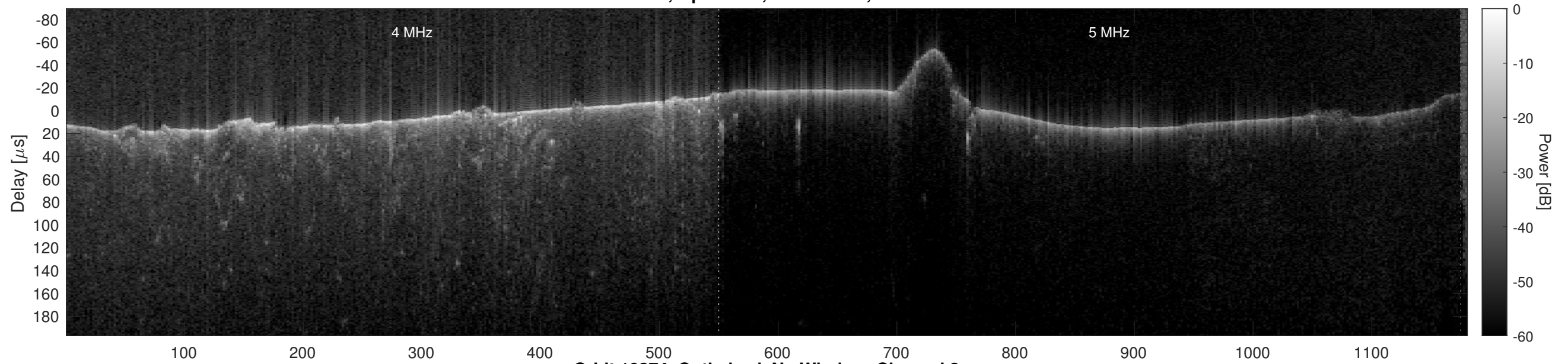
Orbit 10374, Optimized, No Window, Channel 2
