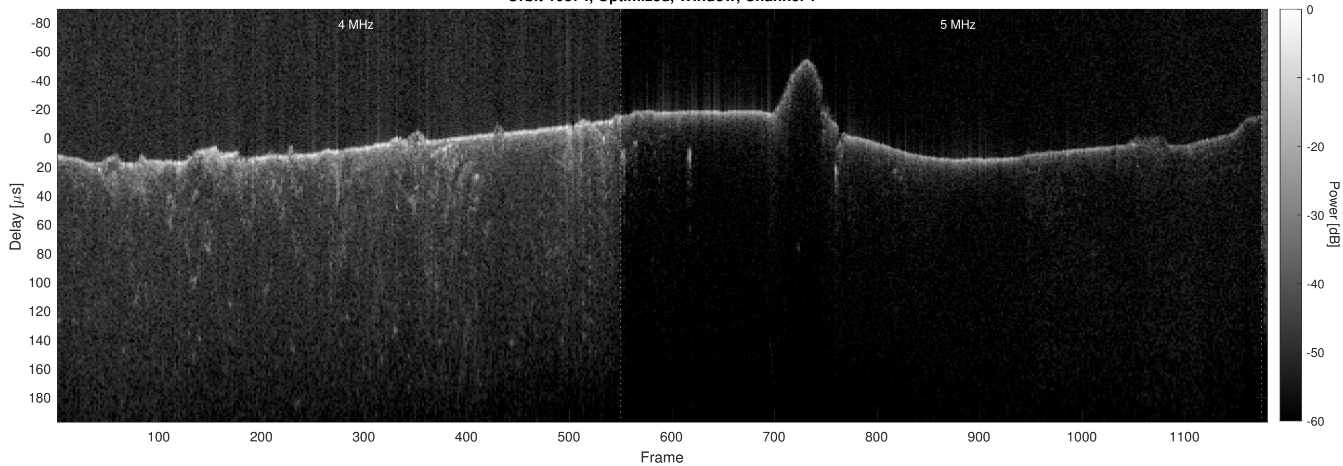
Orbit 10374, Optimized, Window, Channel 2
