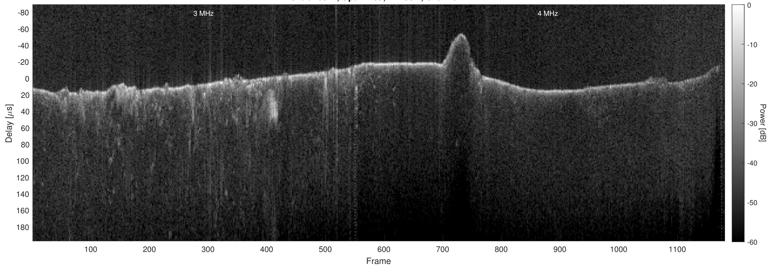
Orbit 10374, Optimized, Window, Channel 2
