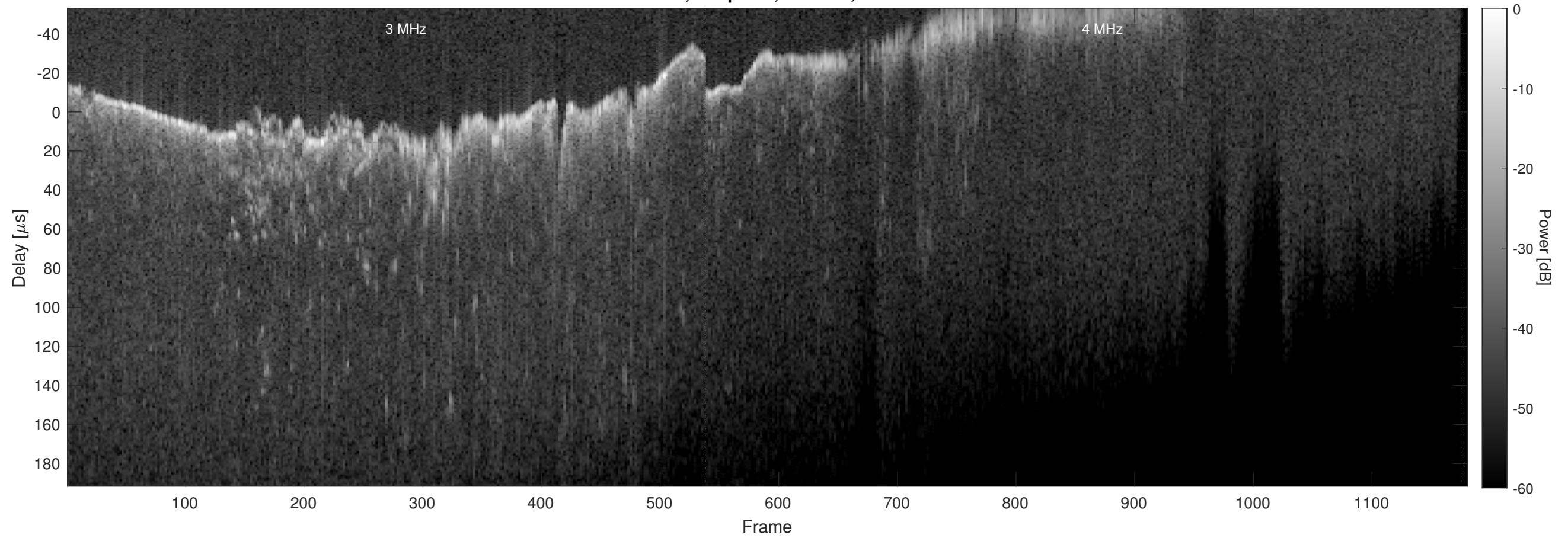
Orbit 10376, Chapman, Window, Channel 2
