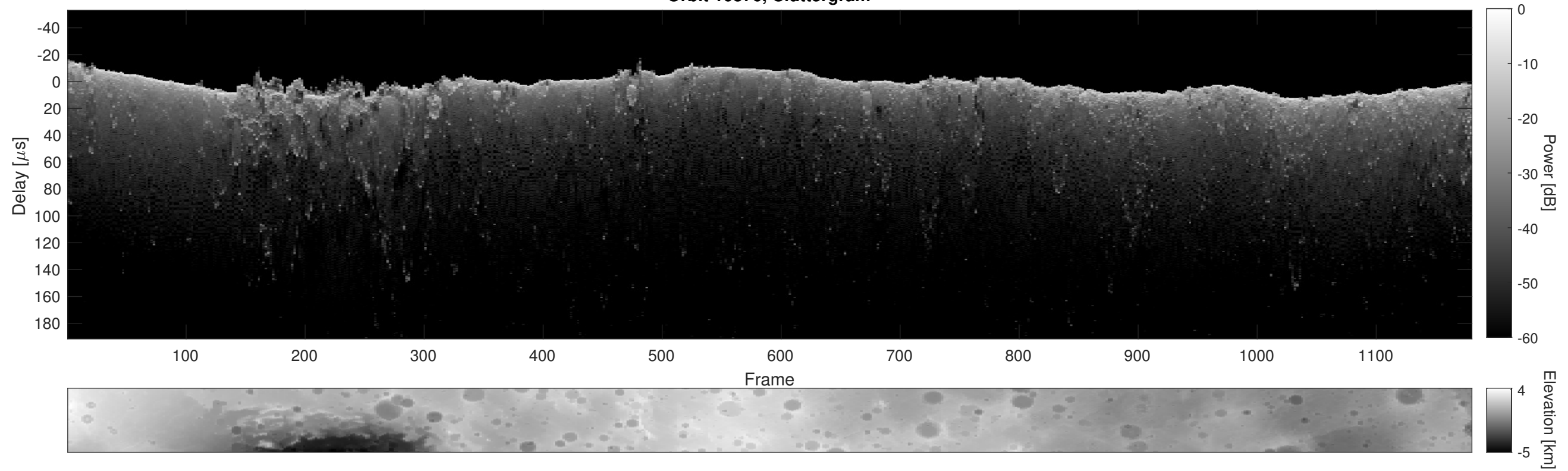
Orbit 10376, Cluttergram
