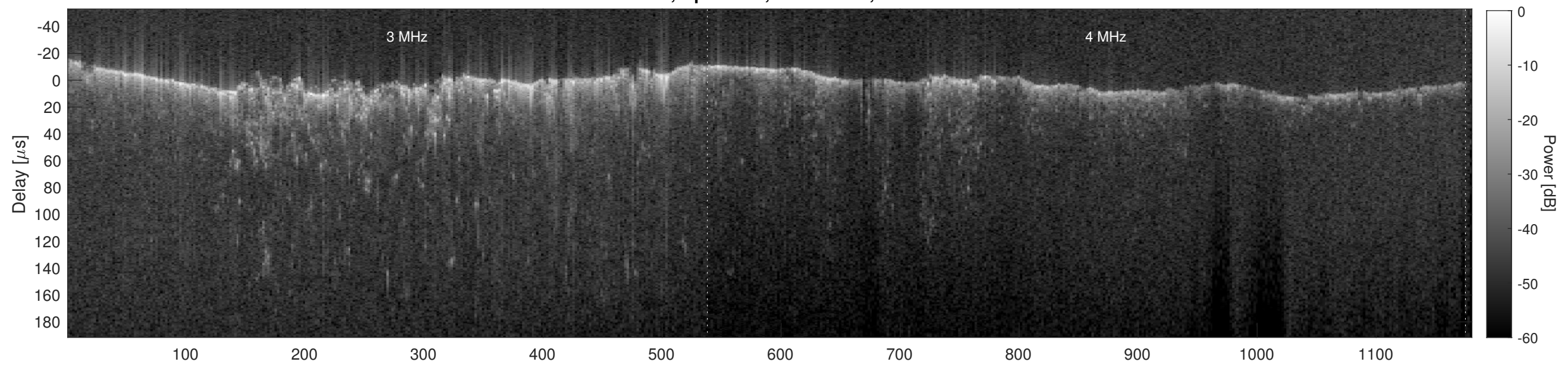
Orbit 10376, Cluttergram
