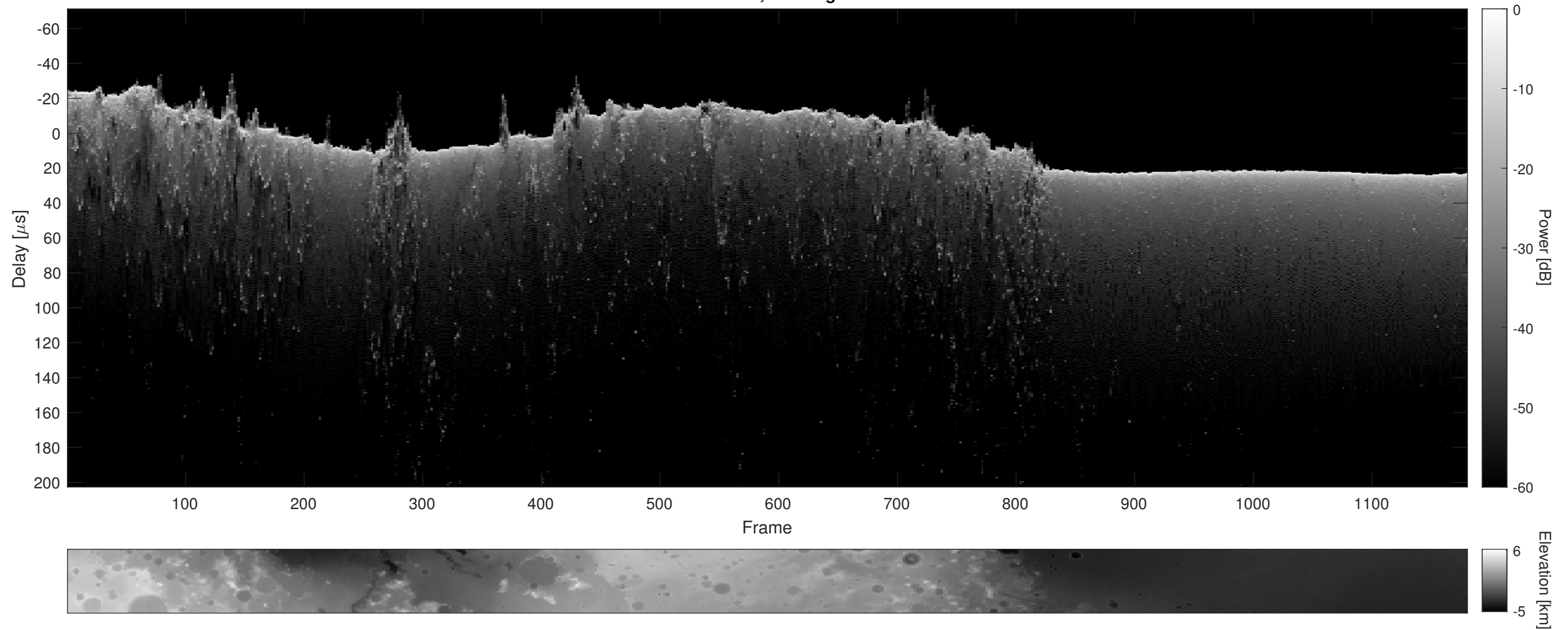
Orbit 10379, Cluttergram
