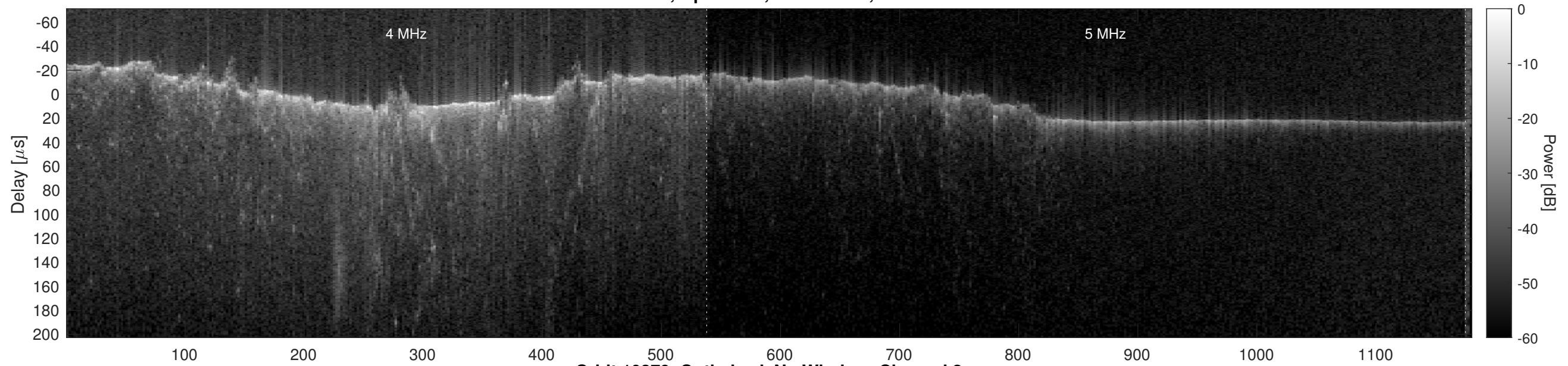
Orbit 10379, Optimized, No Window, Channel 2
