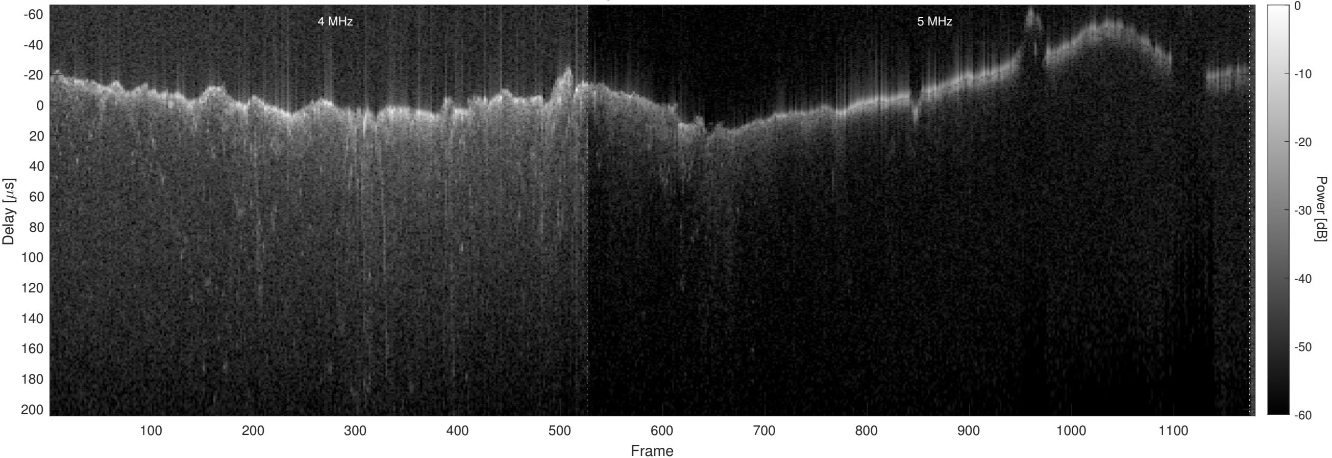
Orbit 10382, Chapman, No Window, Channel 2
