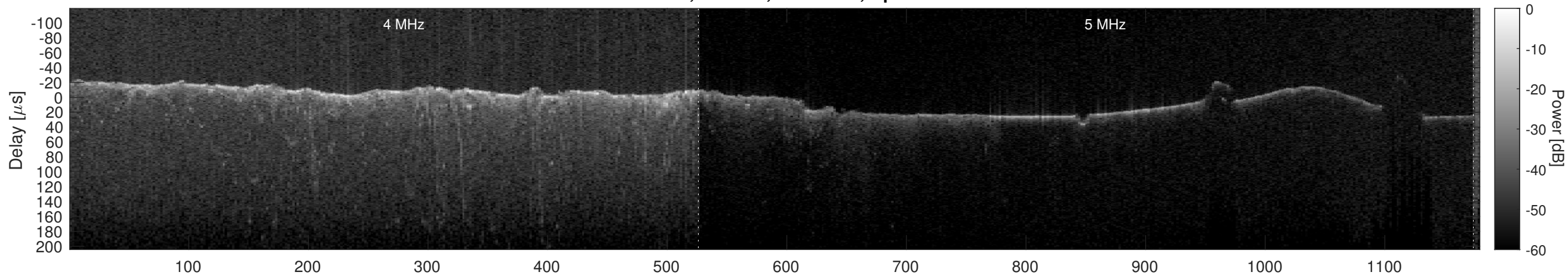
Orbit 10382, Cluttergram
