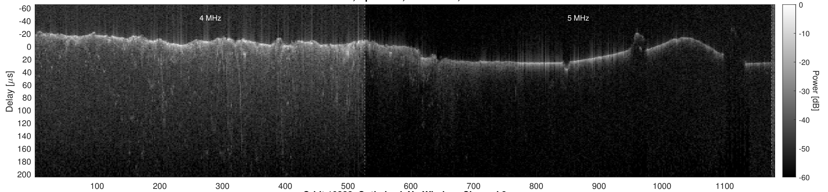
Orbit 10382, Optimized, No Window, Channel 2
