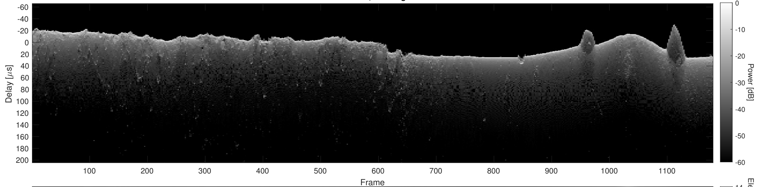
Orbit 10382, Cluttergram
