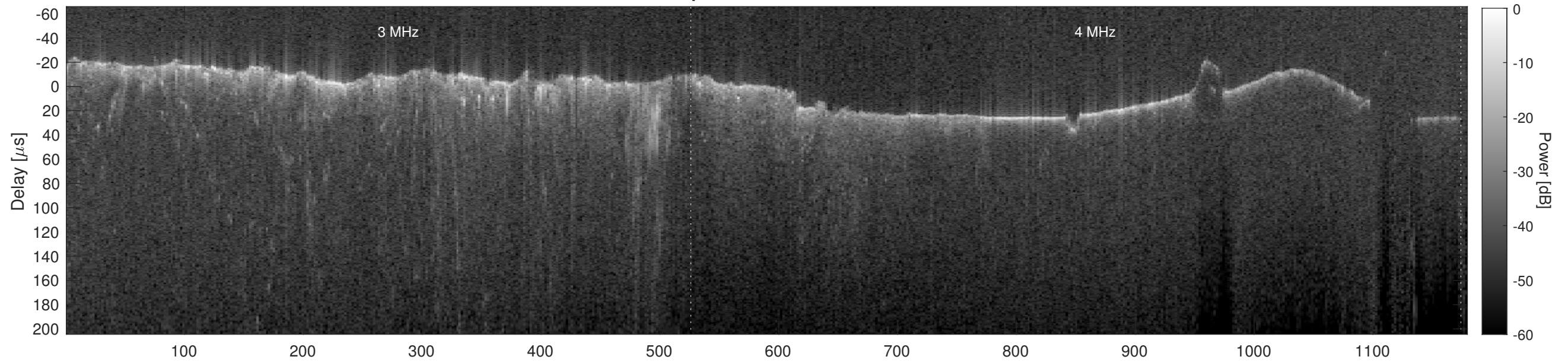
Orbit 10382, Cluttergram
