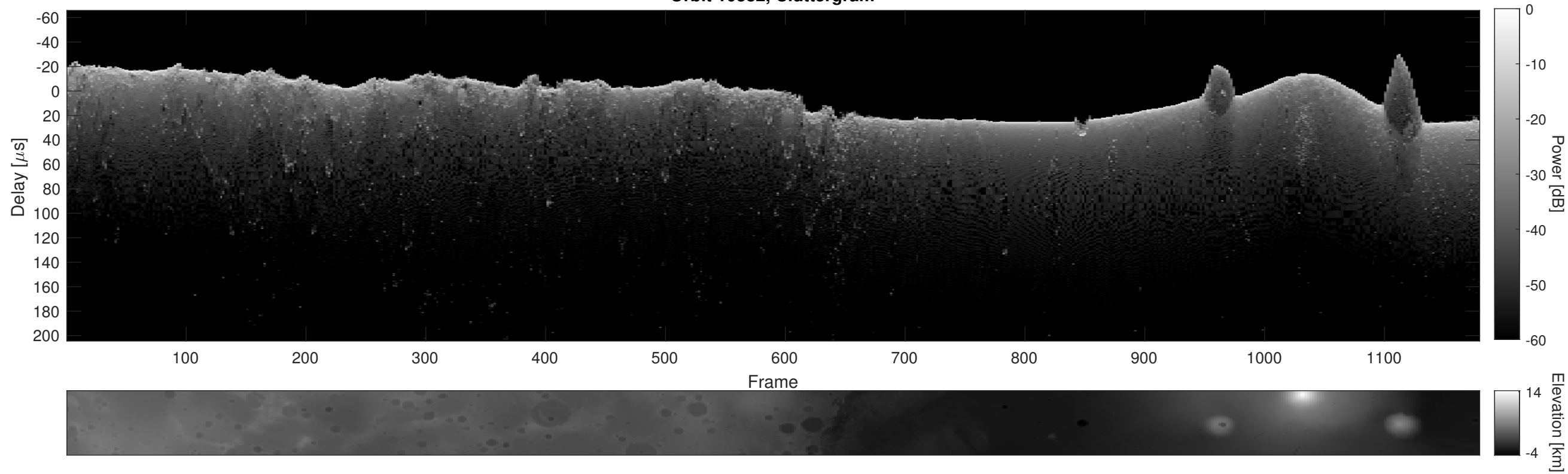
Orbit 10382, Cluttergram
