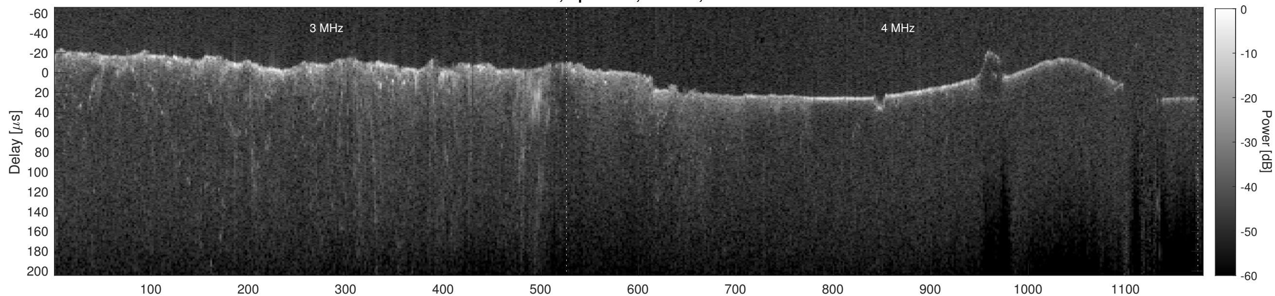
Orbit 10382, Cluttergram
