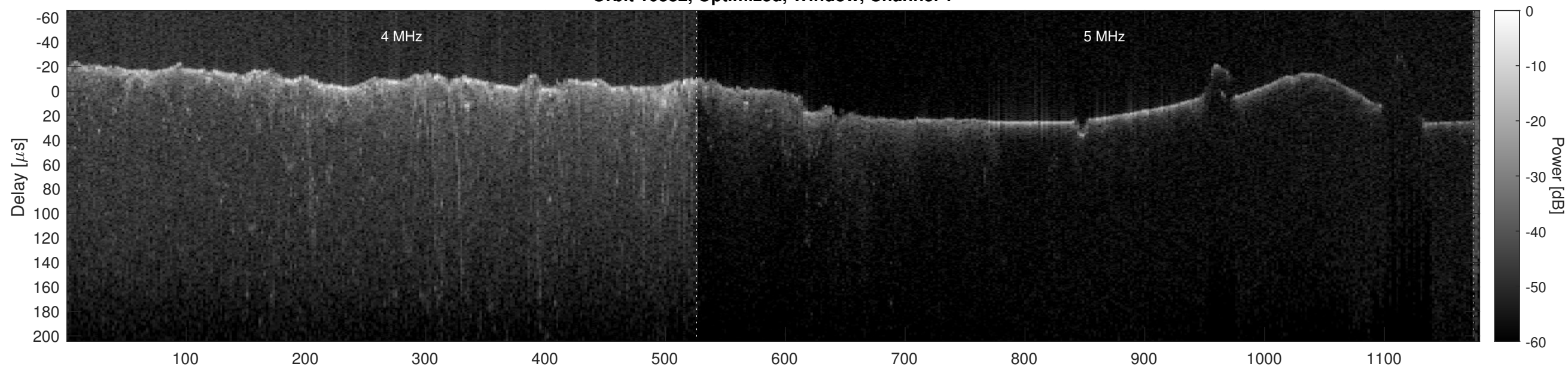
Orbit 10382, Optimized, Window, Channel 2
