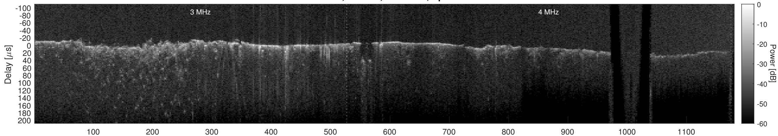
Orbit 10384, Cluttergram
